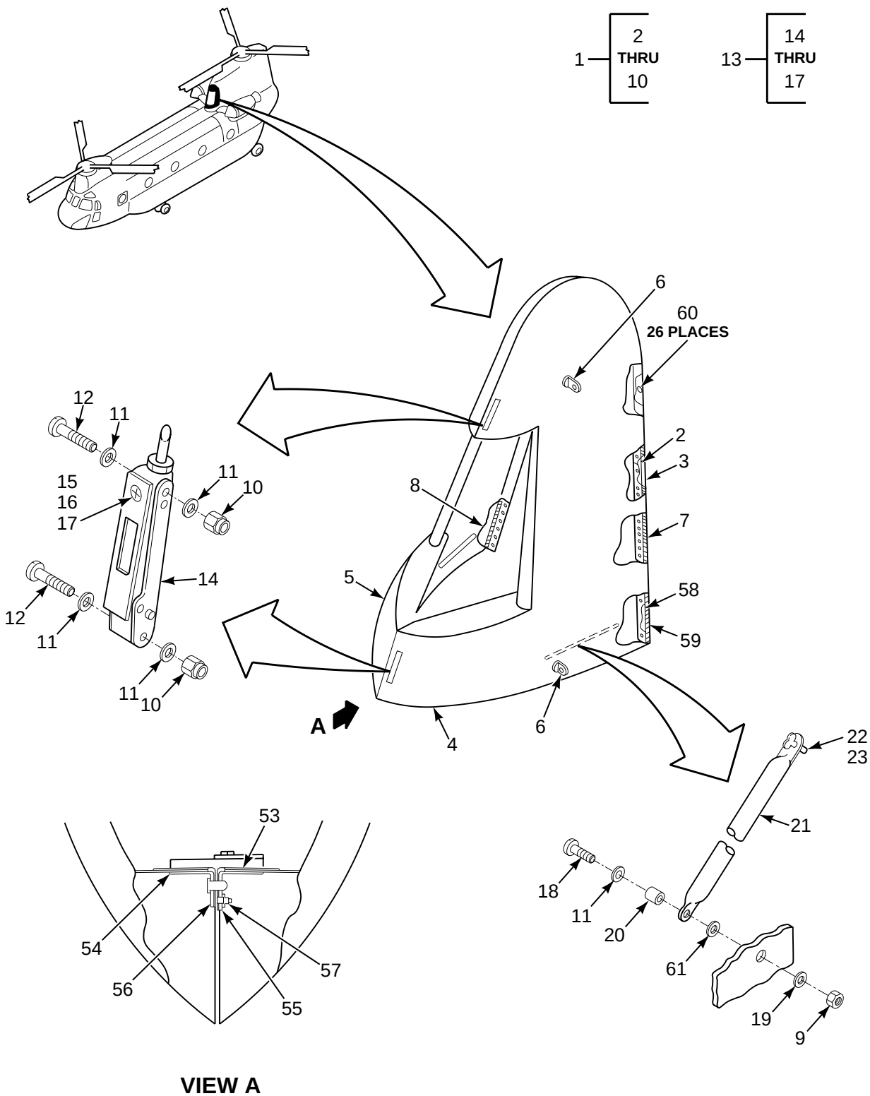
FIGURE 137. FAIRING INSTL, AFT PYLON (SHEET 1 OF 2)
