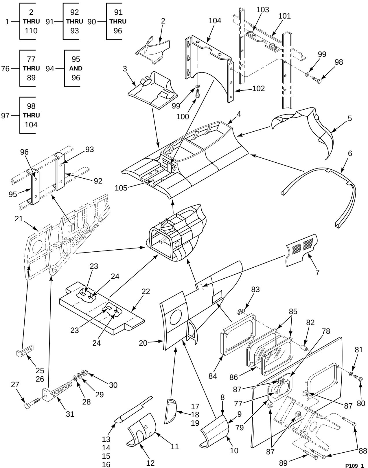
FIGURE 109. STRUCTURE INSTL, AFT FUSELAGE (SHEET 1 OF 4)
