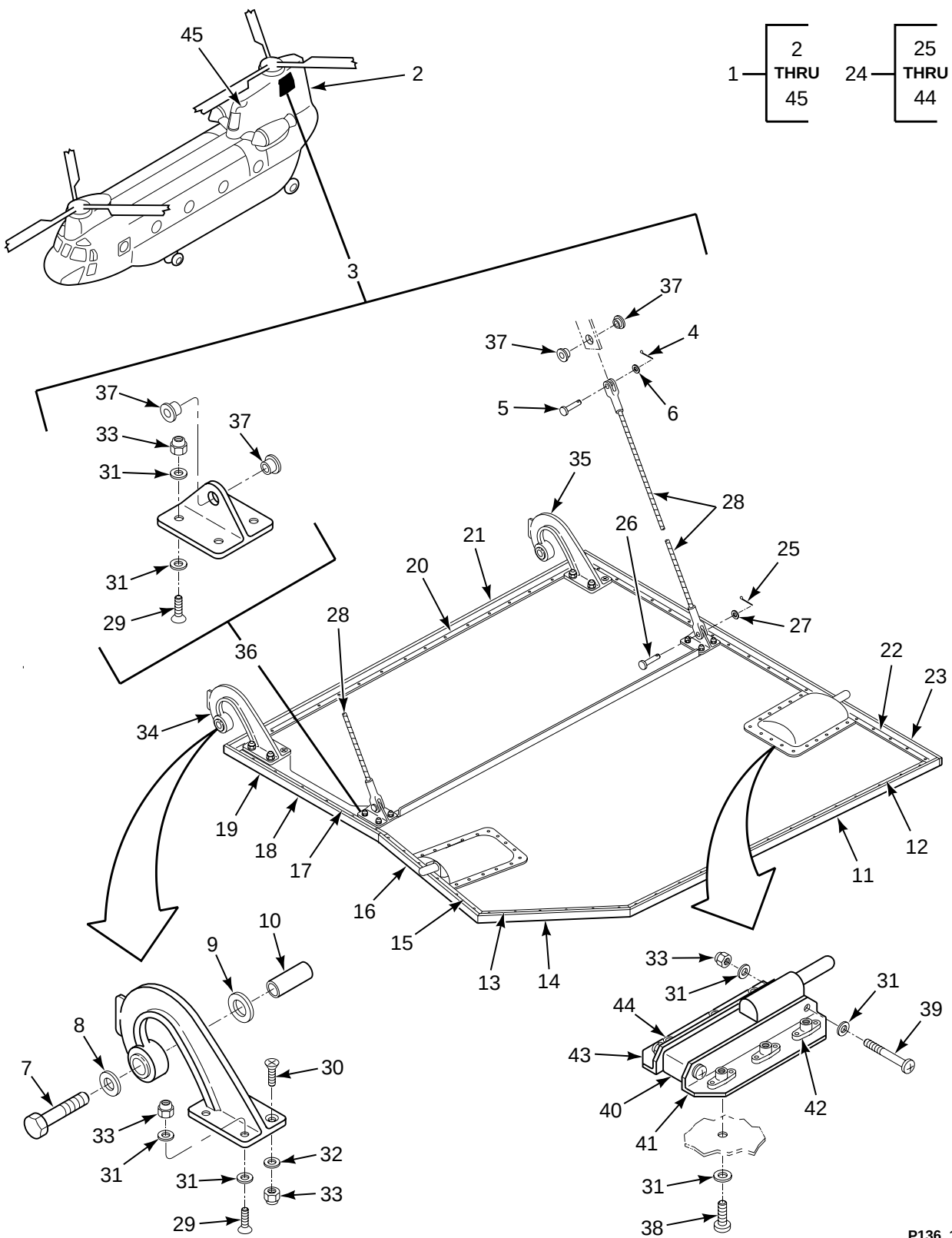
FIGURE 136. PYLON, AFT
