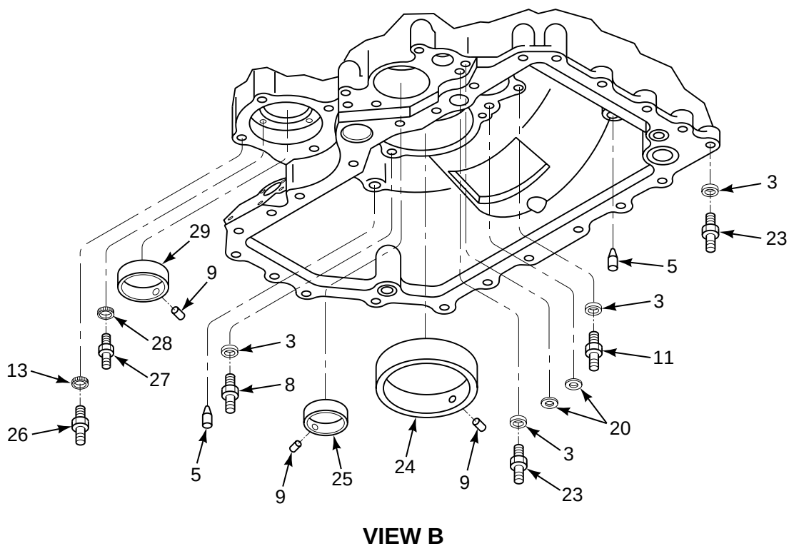
FIGURE 186. HOUSING, MAIN, FWD TRANSMISSION (SHEET 2 OF 2)
