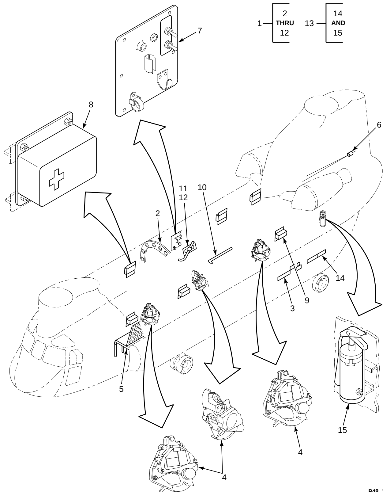
FIGURE 48. EQUIPMENT INSTL, CABIN
