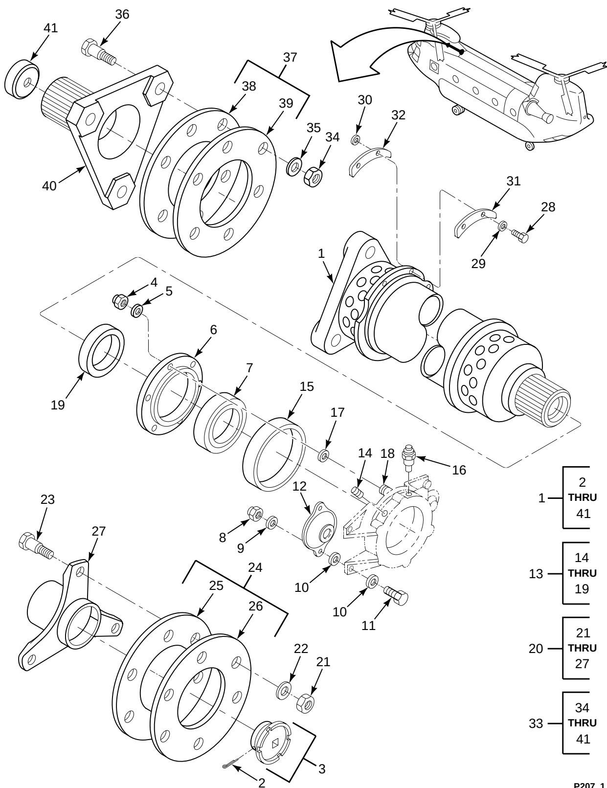
FIGURE 207. SHAFTS, ROTOR DRIVE (SHEET 1 OF 7)
