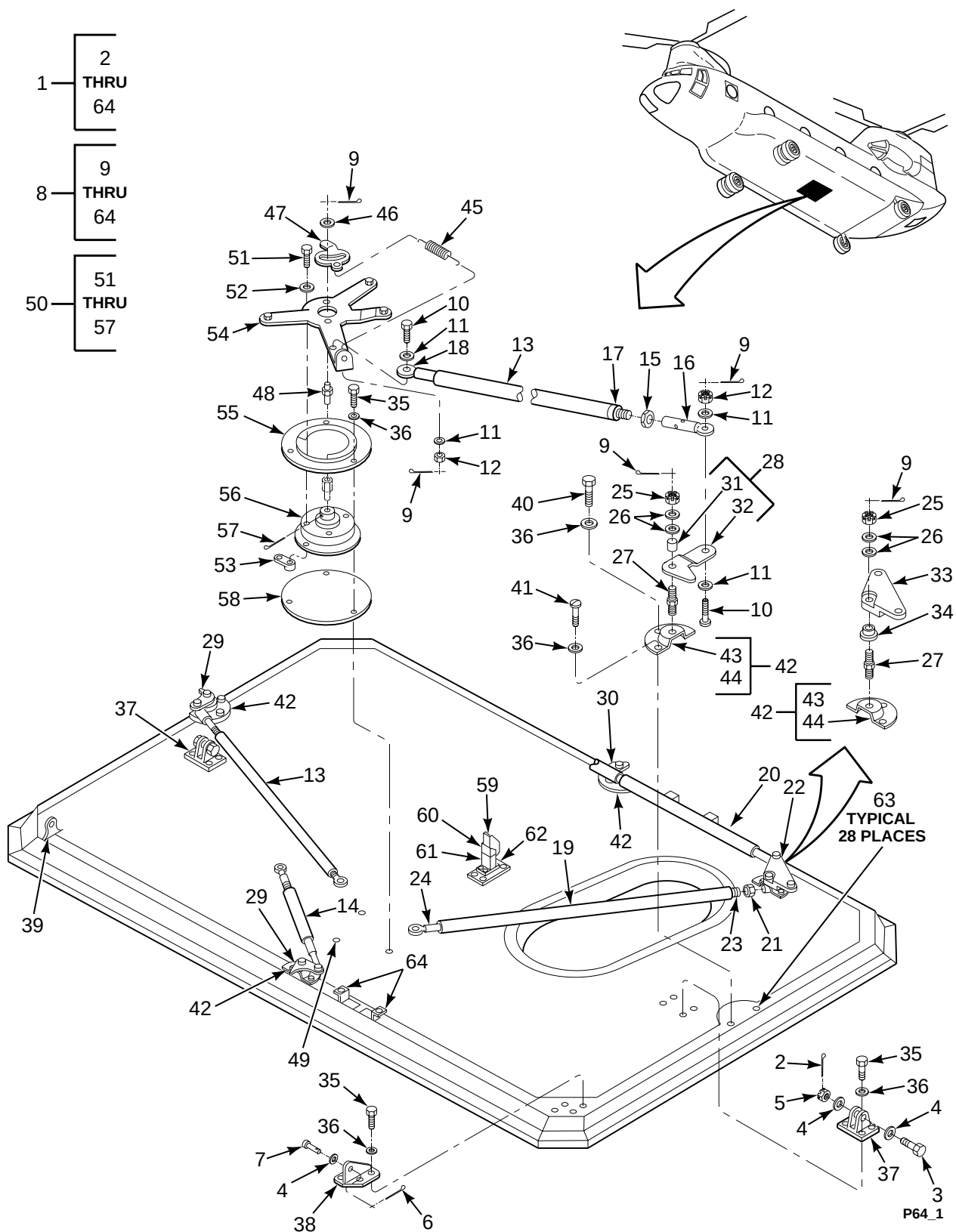
FIGURE 64. DOOR INSTL, RESCUE
