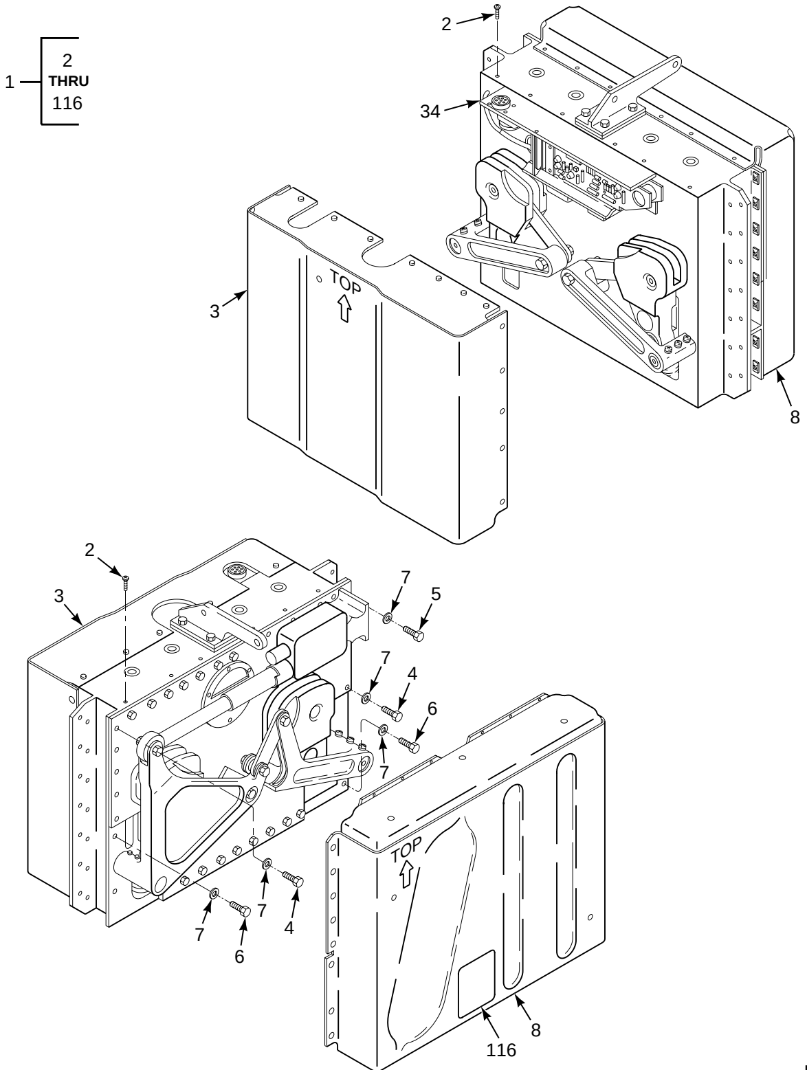
FIGURE 28. ABSORBER, VIBRATION, SELF-TUNING (SHEET 1 OF 5)
