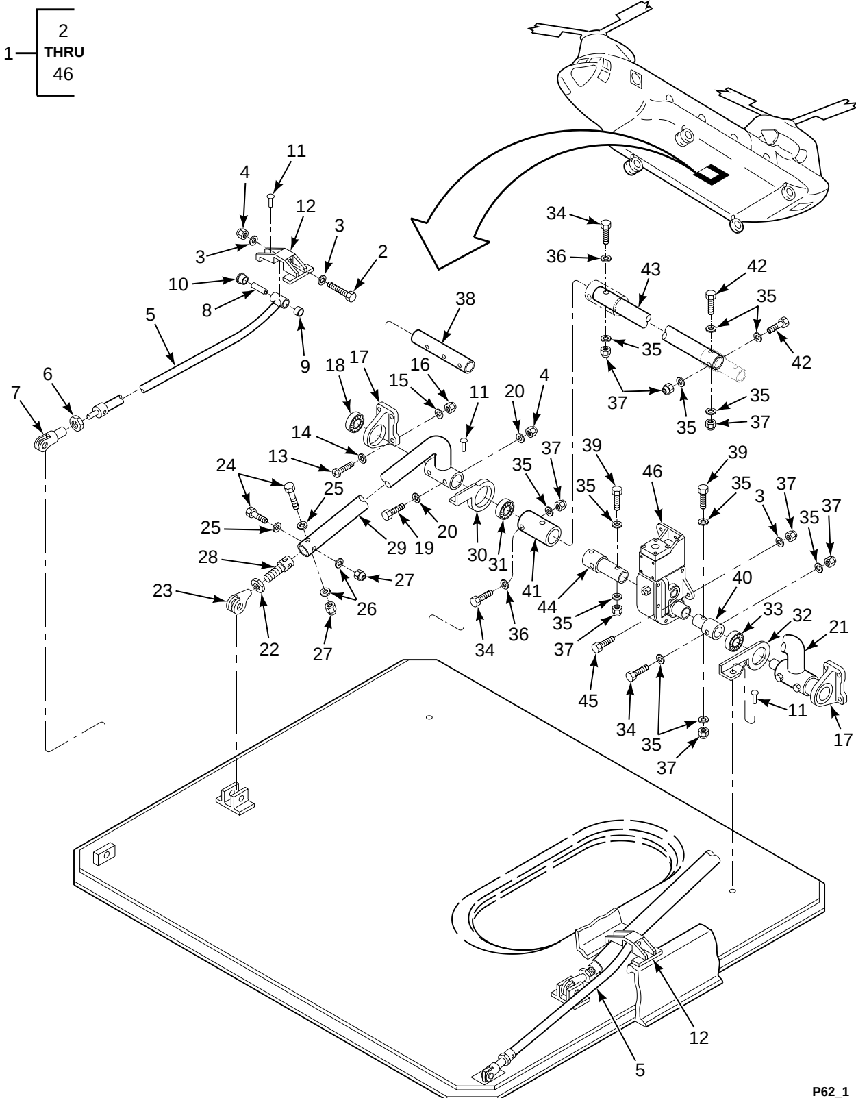
FIGURE 62. ACTUATOR MECHANISM INSTL, DOOR, LOWER RESCUE HATCH
