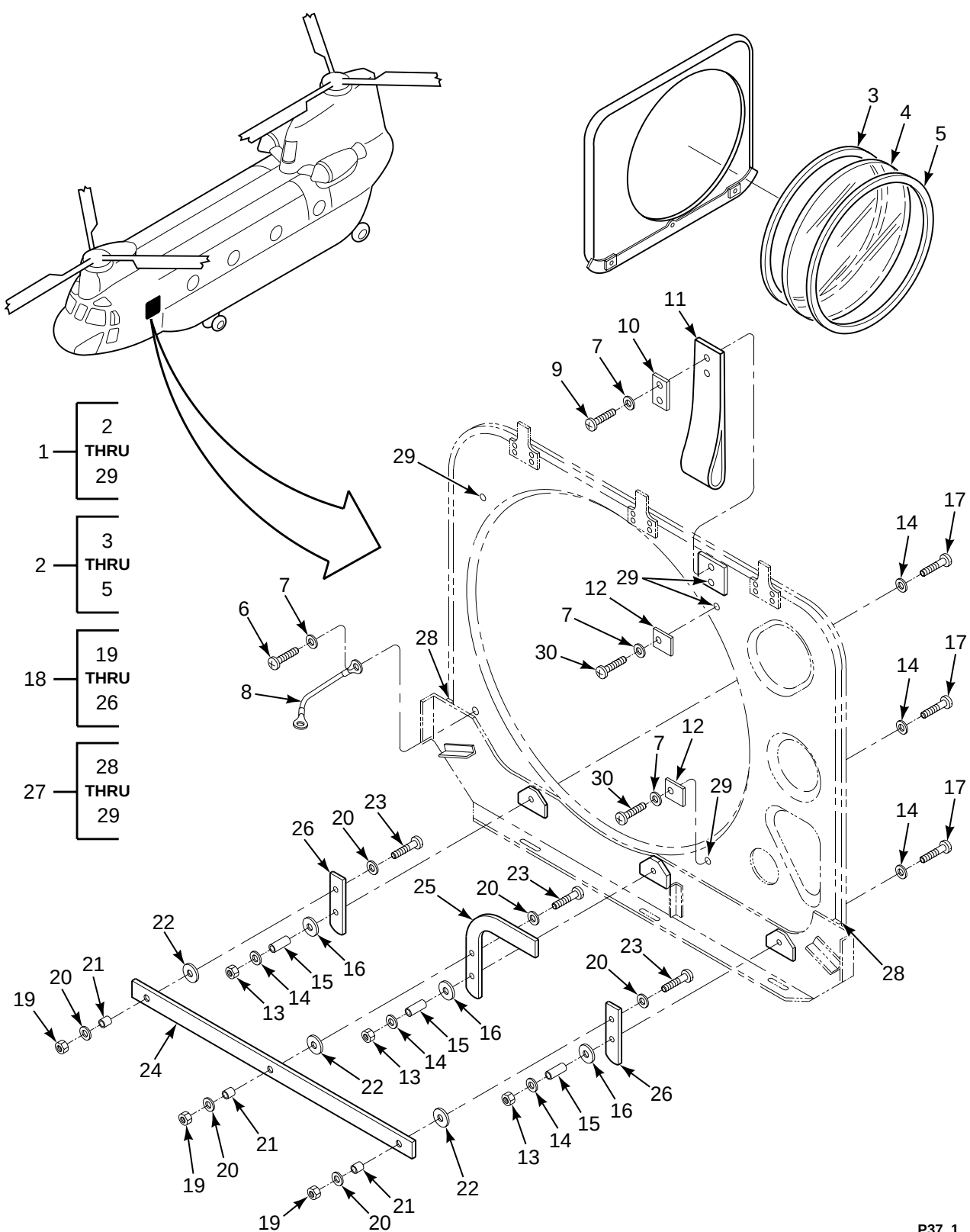
FIGURE 37. HATCH ASSY, REPLACEABLE ESCAPE, CABIN LH
