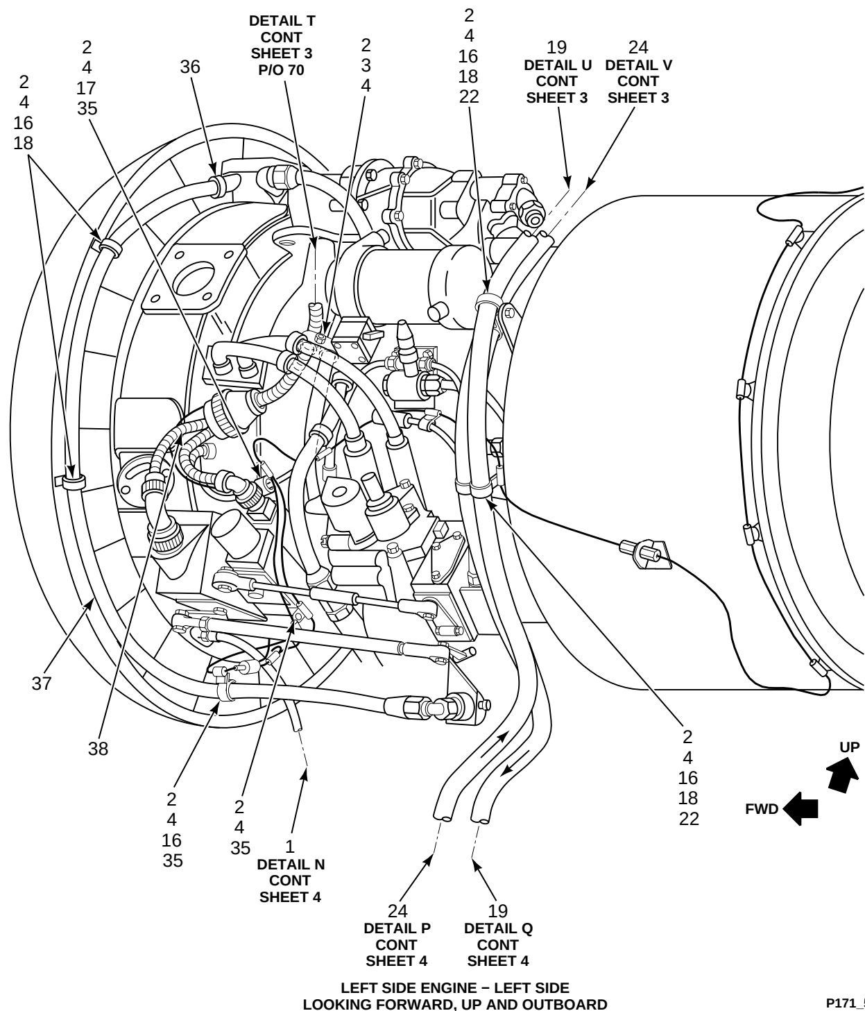
FIGURE 171. TUBING AND WIRING INSTL (T55-L-712 ENGINE) (SHEET 5 OF 6)
