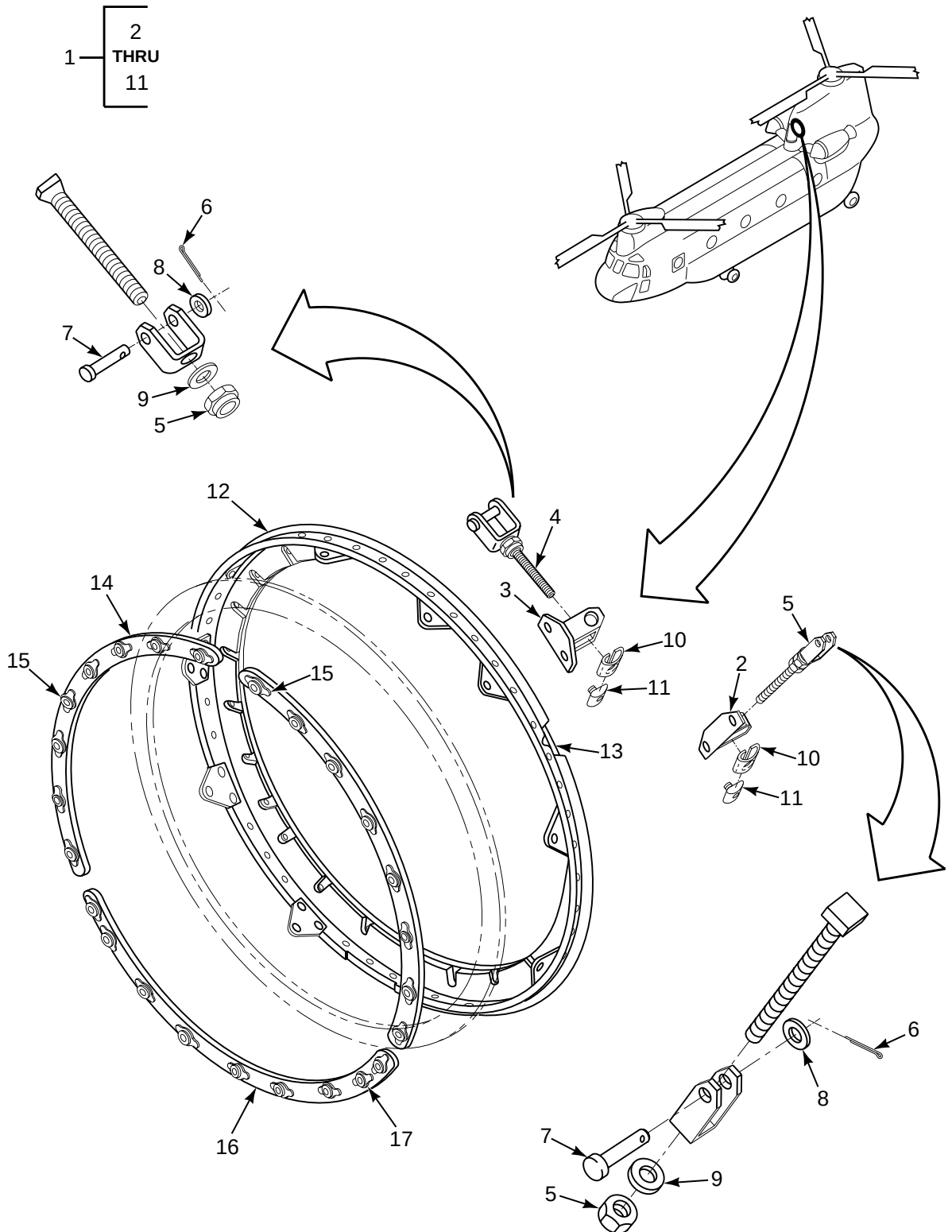
FIGURE 166. BRACKET, FORMER, AND RING ASSEMBLIES
