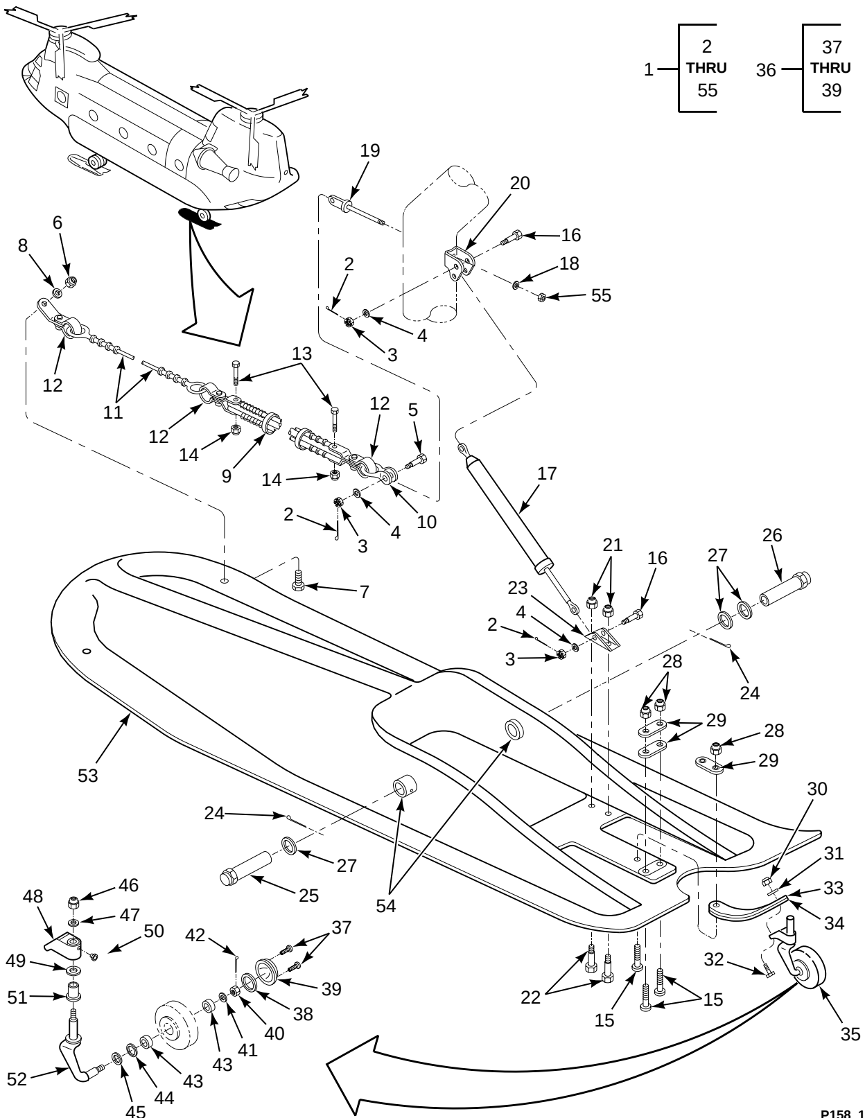
FIGURE 158. SKI ASSEMBLY, LANDING GEAR, AFT
