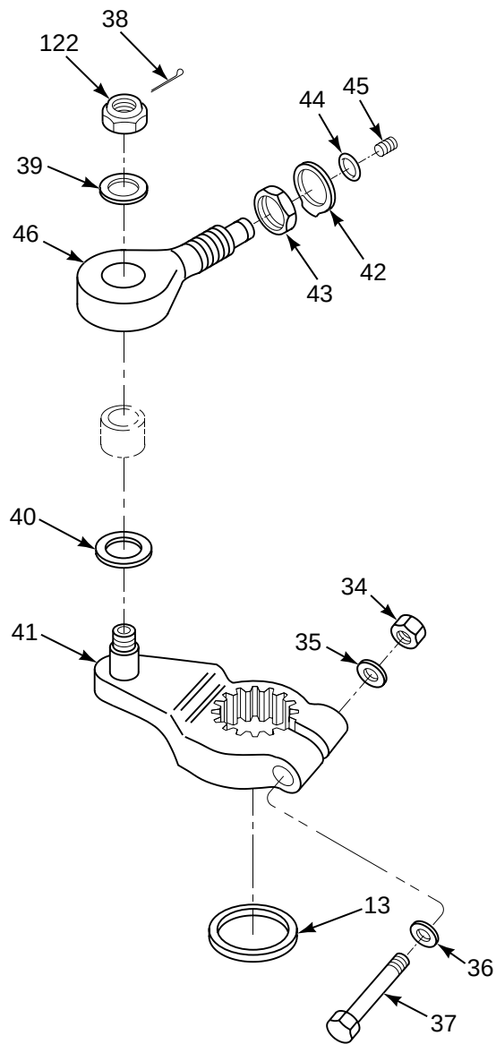
DETAIL C
