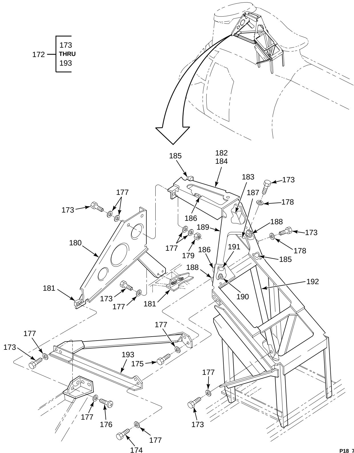
FIGURE 18. STRUCTURE, COCKPIT (SHEET 7 OF 7)
