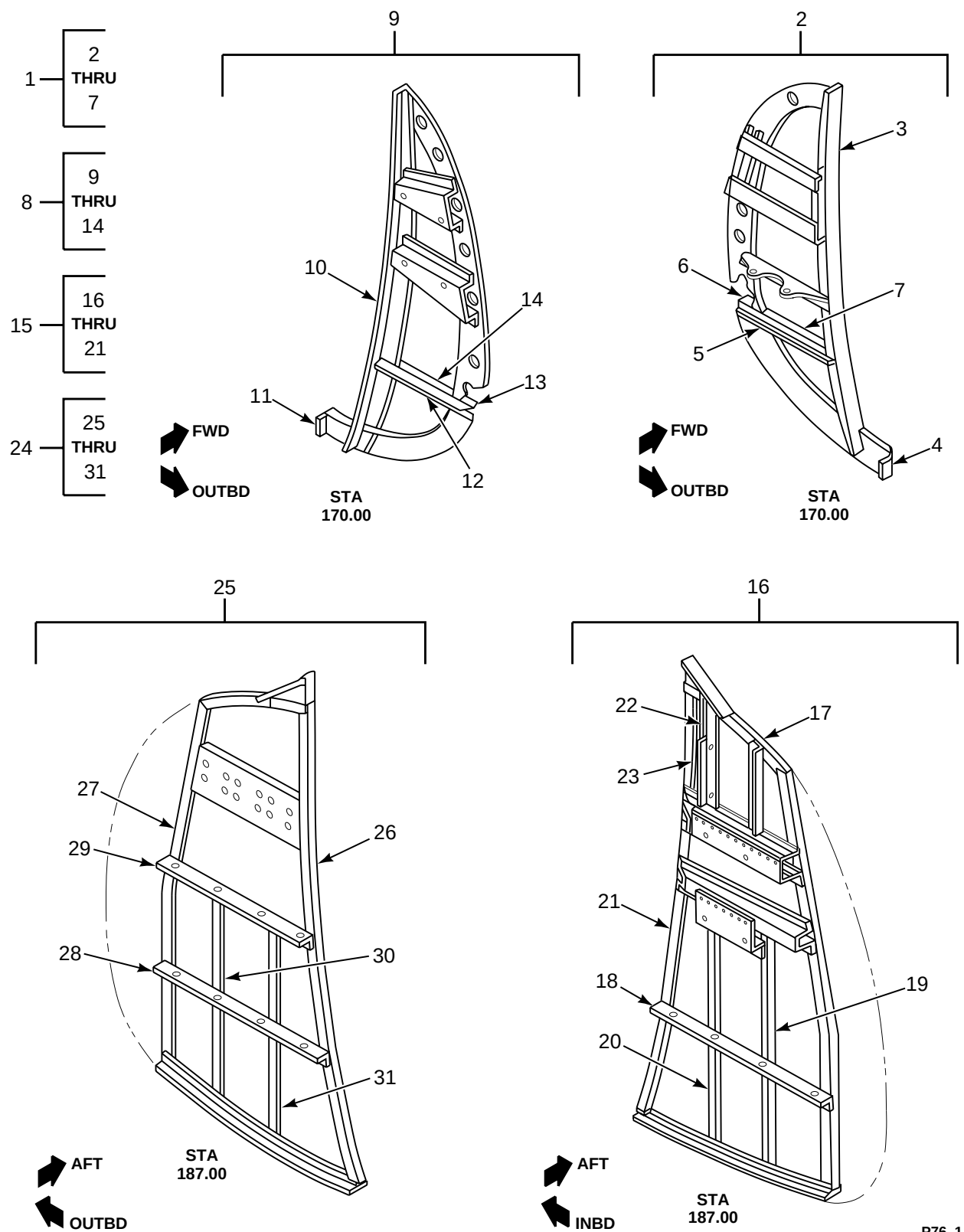
FIGURE 76. FORMER INSTL, STA 170, LH AND RH
