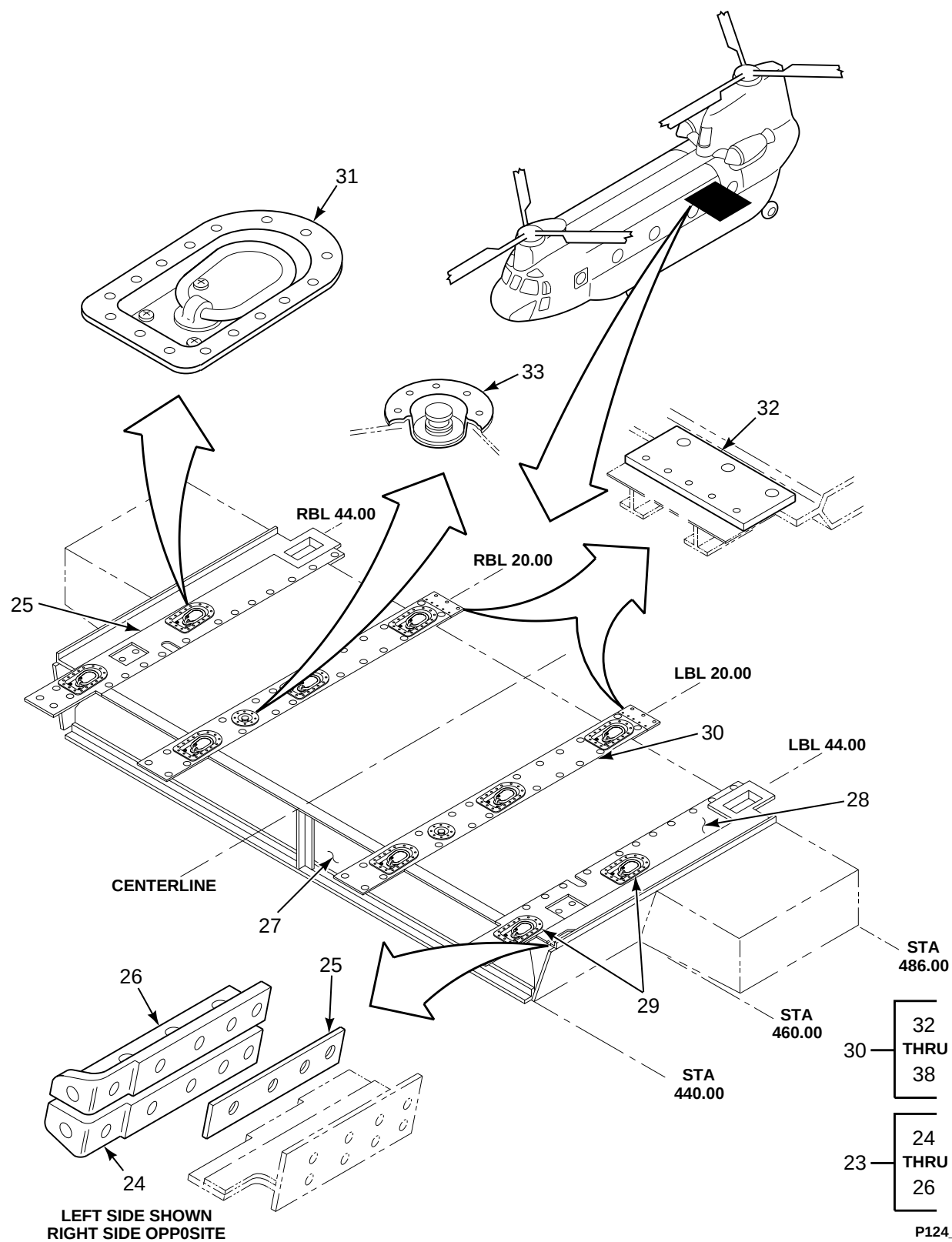
FIGURE 124. PANEL, LOWER AFT FUSELAGE (SHEET 2 OF 2)
