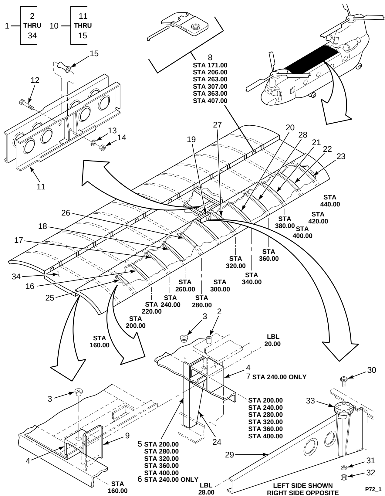
FIGURE 72. CROWN, CABIN
