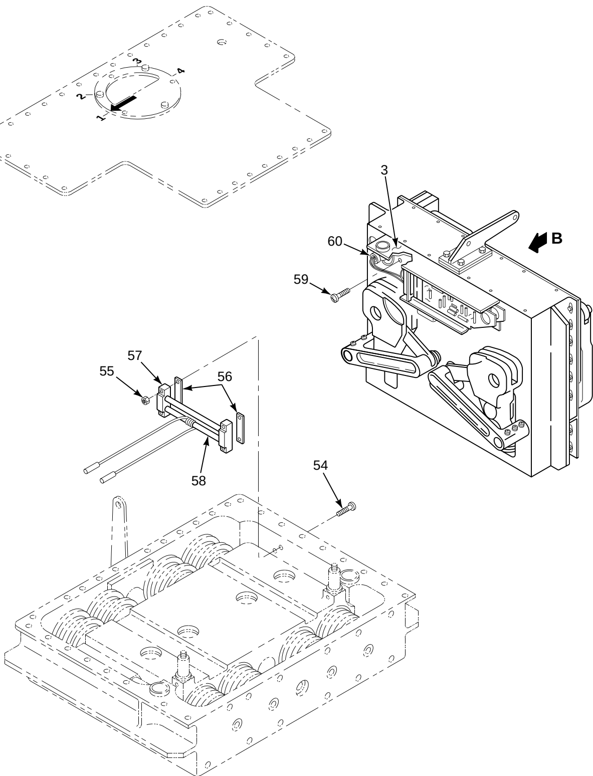
VIEW B
