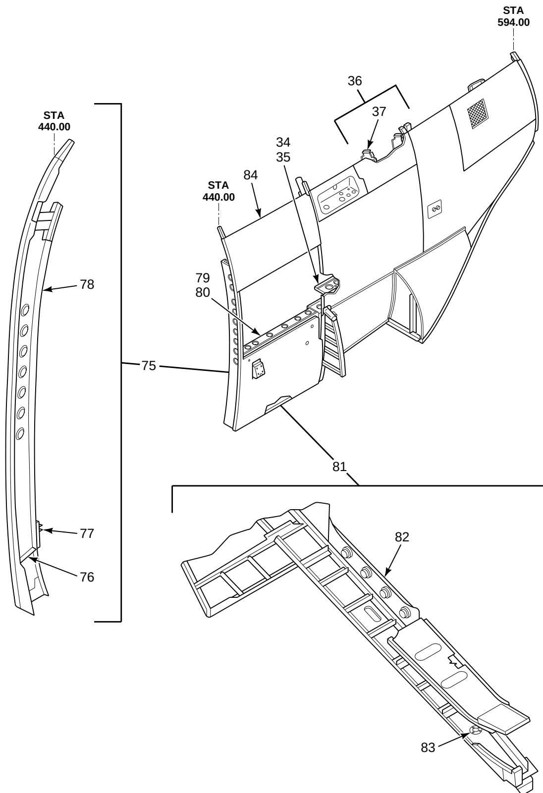
FIGURE 133. PANEL, STA 440.00 TO 594.00, LH AND RH (SHEET 4 OF 4)
