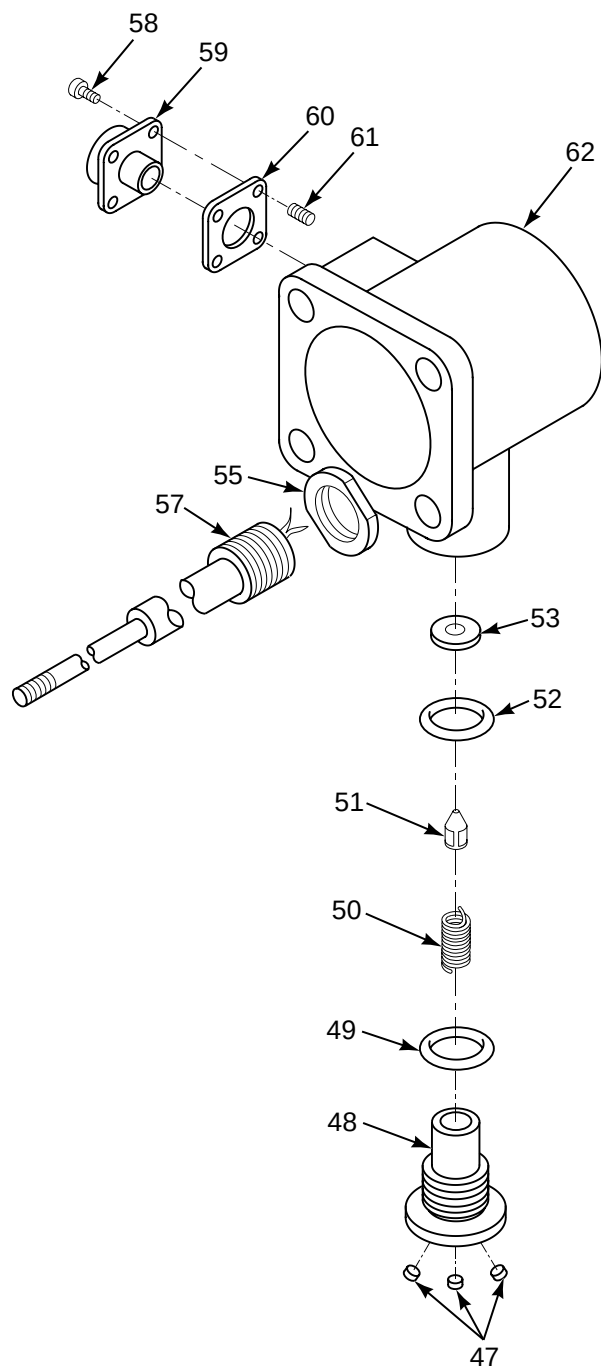
DETAIL D
