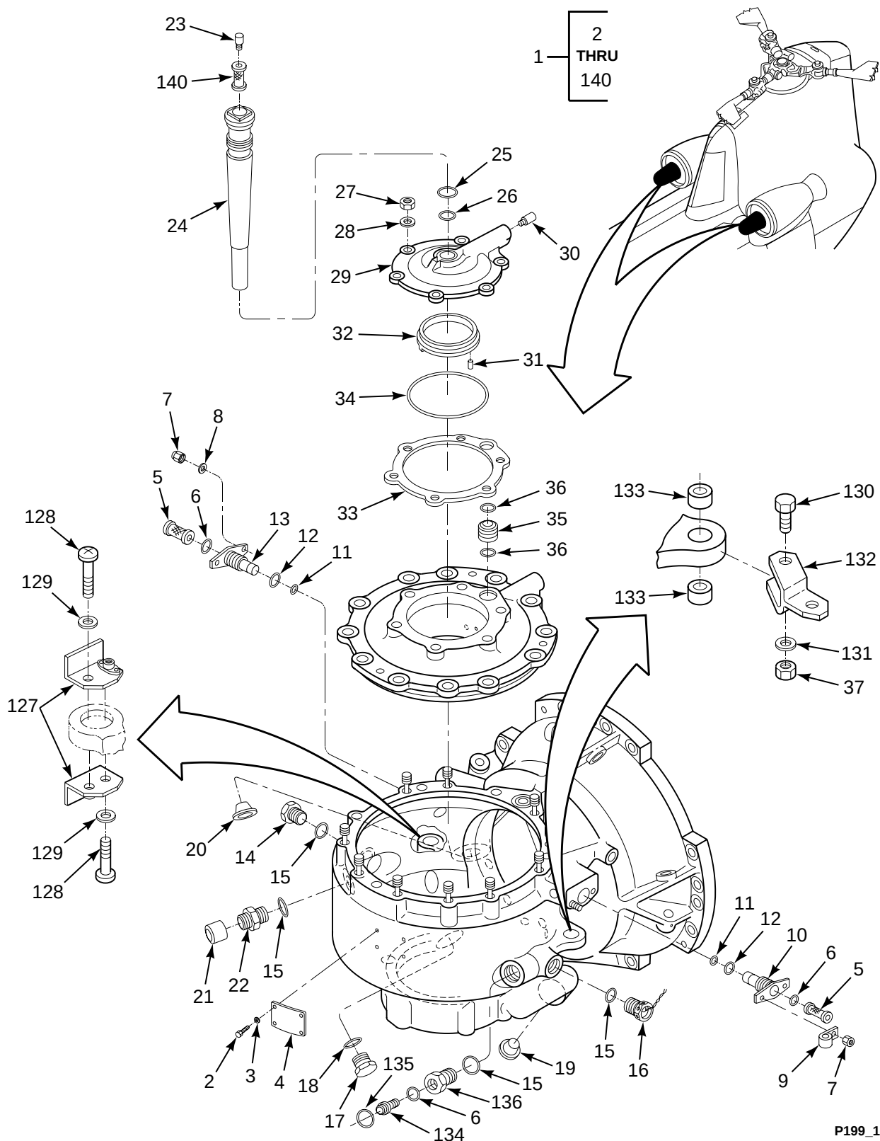
FIGURE 199. TRANSMISSION, ENGINE (SHEET 1 OF 3)
