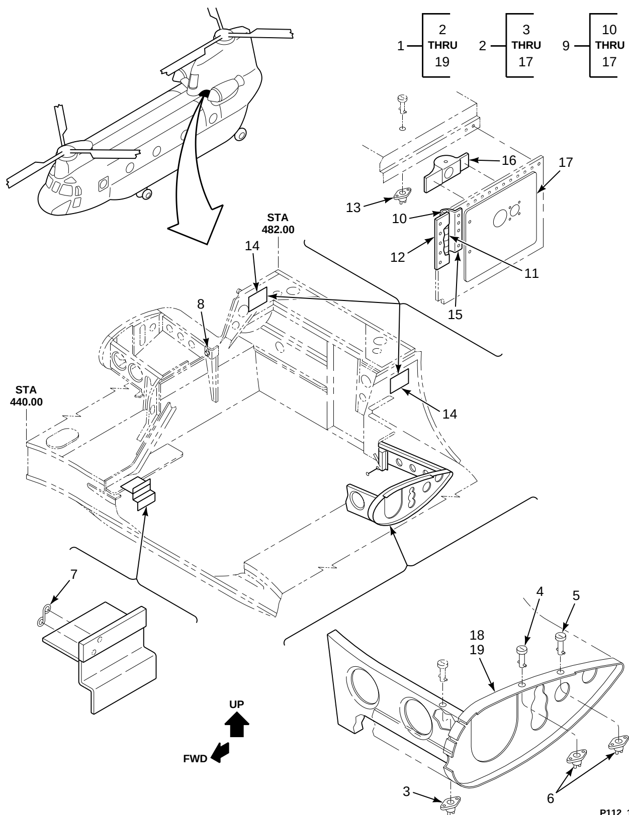
FIGURE 112. FAIRING INSTL, FIXED LOWER PYLON LEADING EDGE
