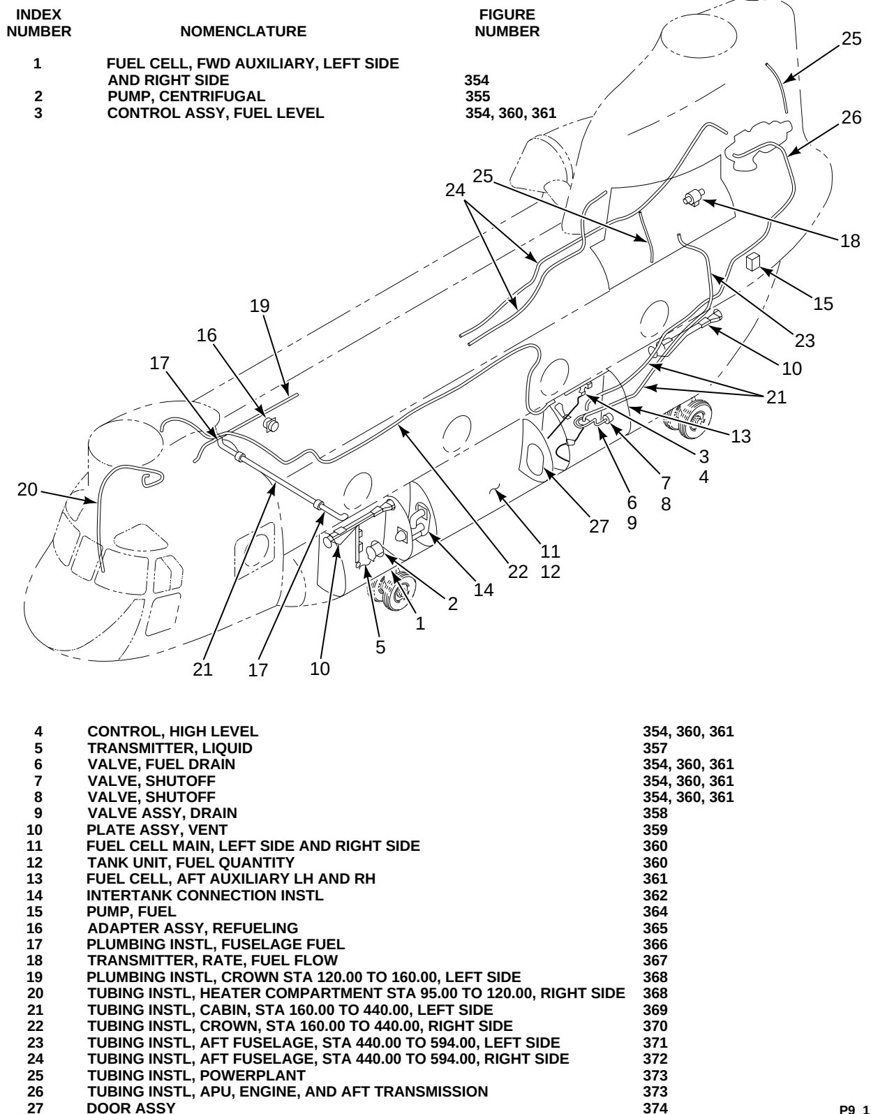
FIGURE 9. FUEL SYSTEM
