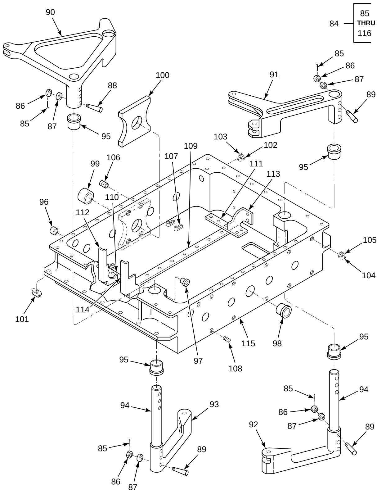
FIGURE 28. ABSORBER, VIBRATION, SELF-TUNING (SHEET 5 OF 5)
