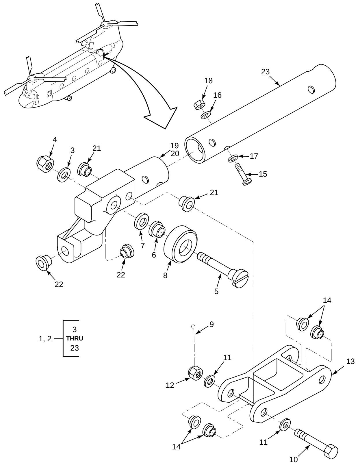
FIGURE 106. TROLLEY, FWD, LH AND RH
