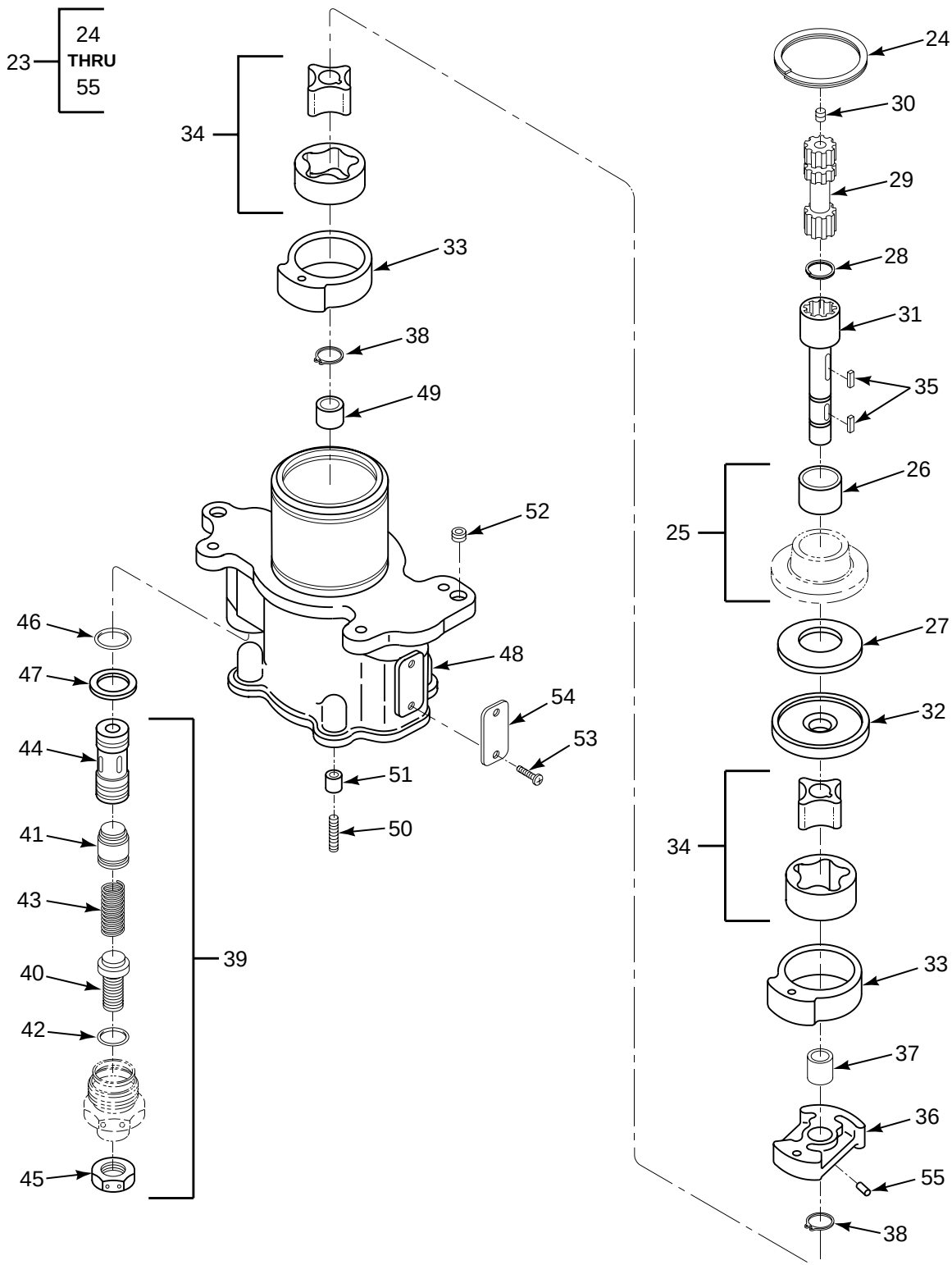
FIGURE 187. PUMPS, LUBE, FWD TRANSMISSION (SHEET 2 OF 2)
