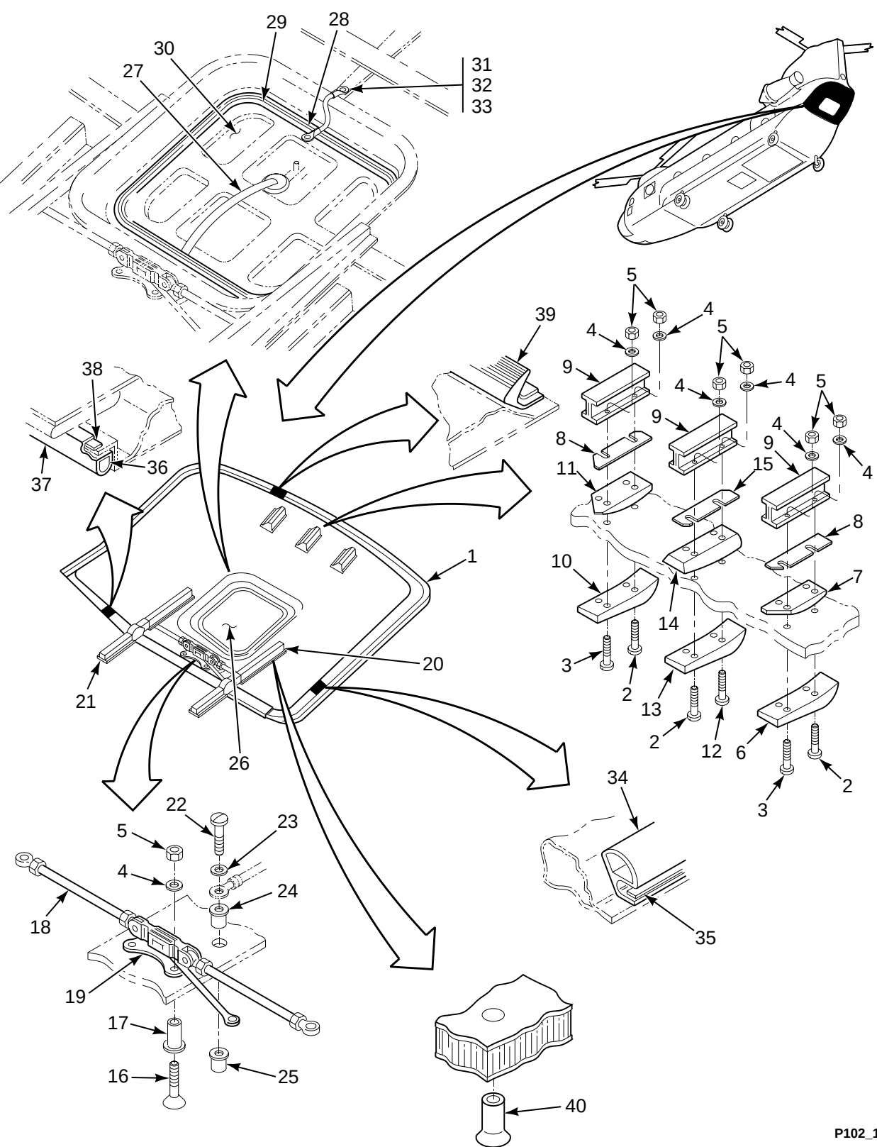
FIGURE 102. DOOR, CARGO
