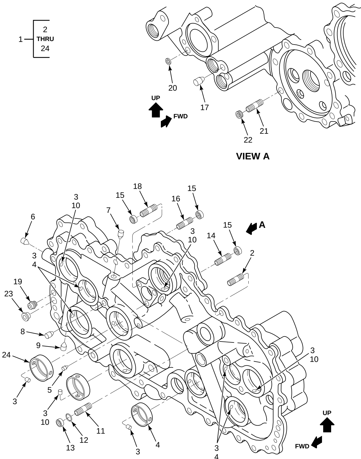
FIGURE 192. HOUSING, ACCESSORY, AFT TRANSMISSION
