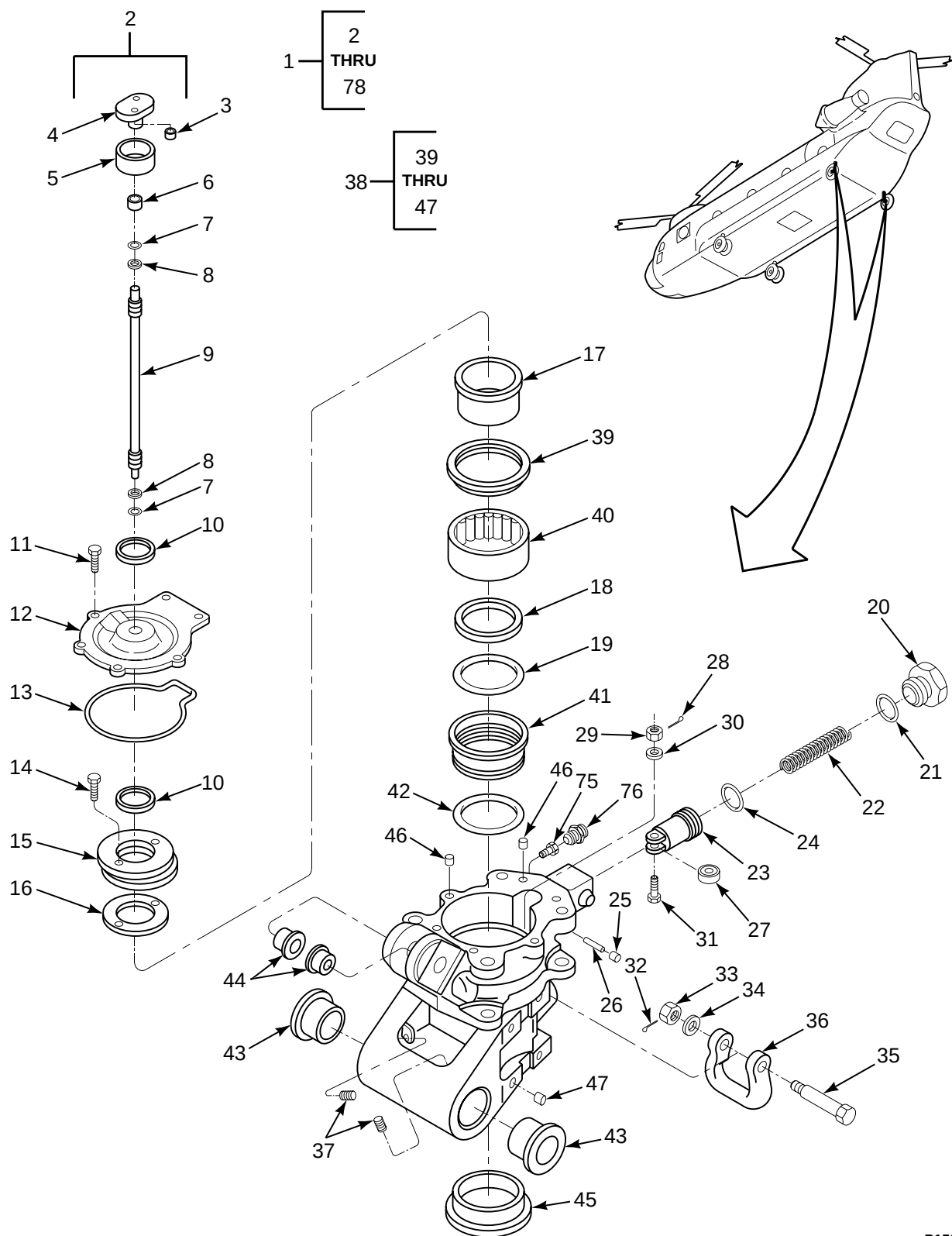
FIGURE 152. HOUSING, SWIVEL, AFT LANDING GEAR (SHEET 1 OF 2)
