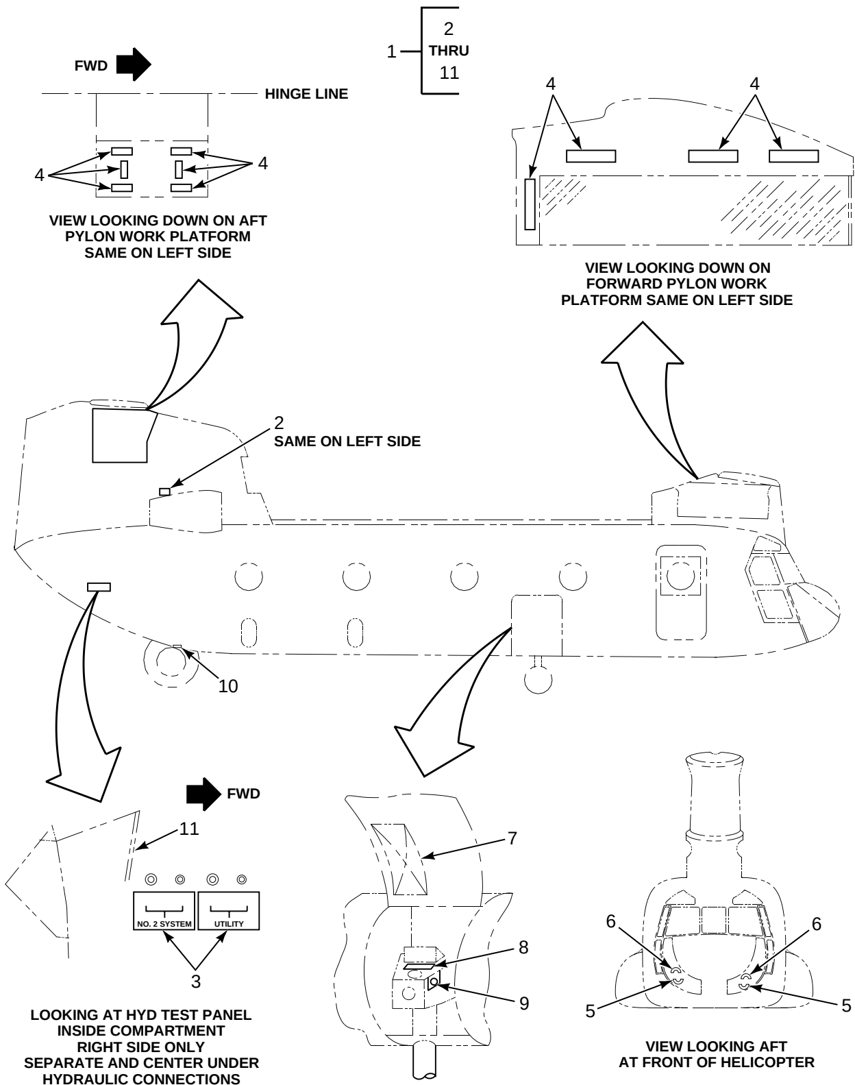
FIGURE 55. MARKINGS, EXTERIOR
