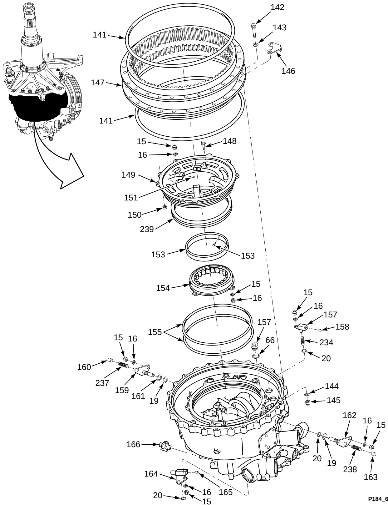
FIGURE 184. TRANSMISSION, FWD (SHEET 6 OF 9)
