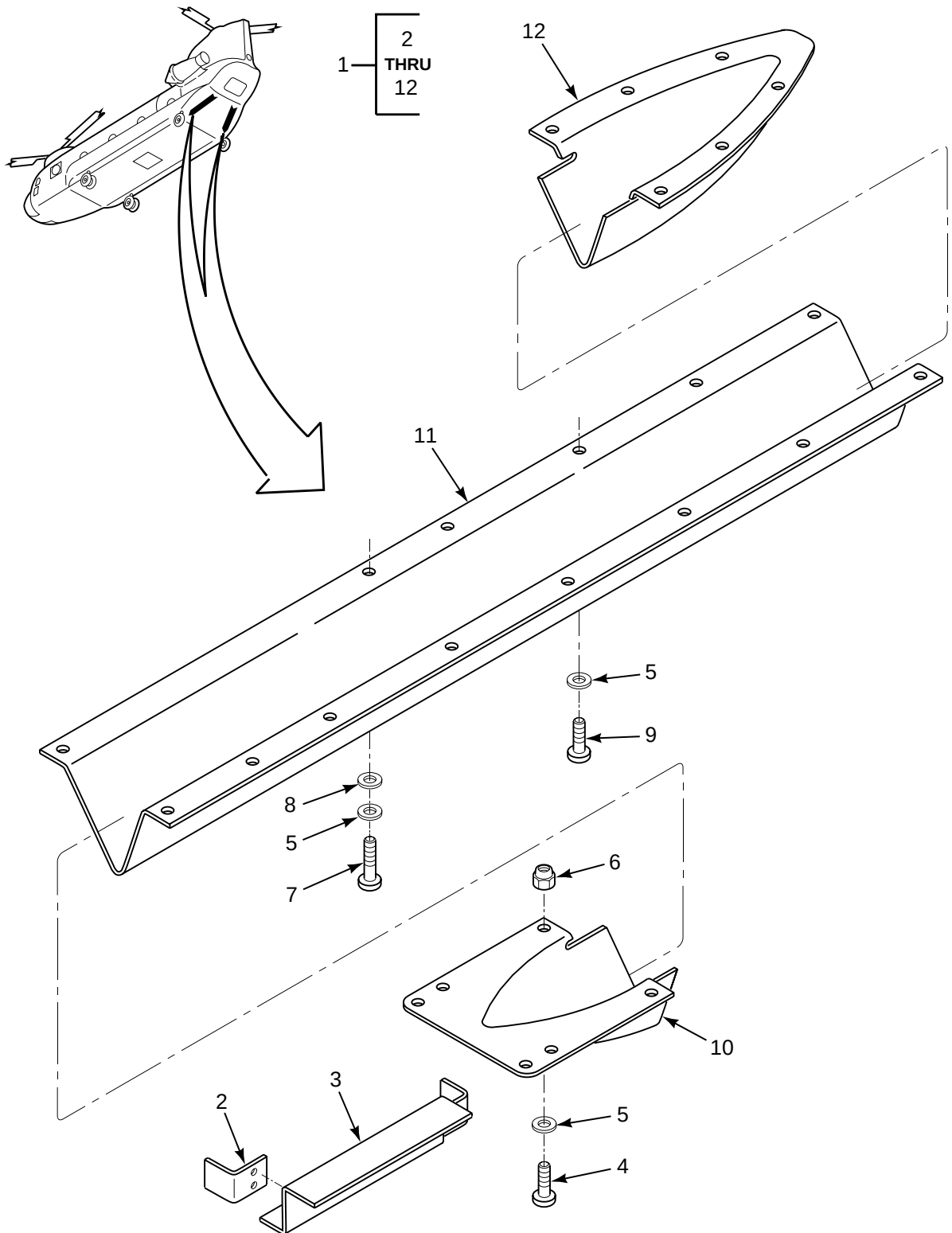
FIGURE 101. STRAKE INSTL, RAMP, LH AND RH
