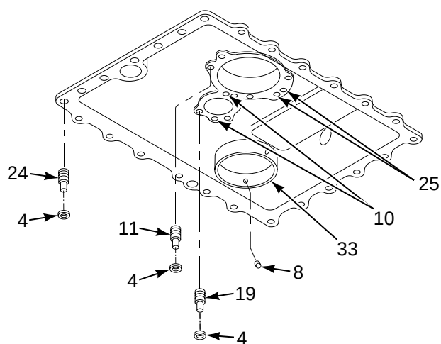
VIEW A
