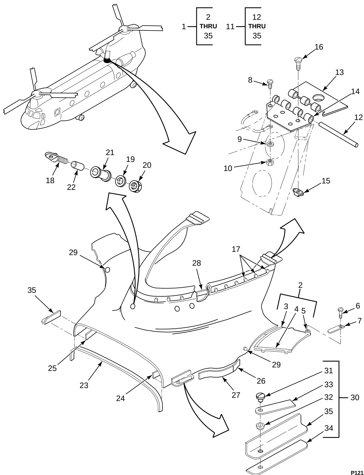
FIGURE 121. FAIRING INSTL, HINGED, LOWER PYLON, LEADING EDGE
