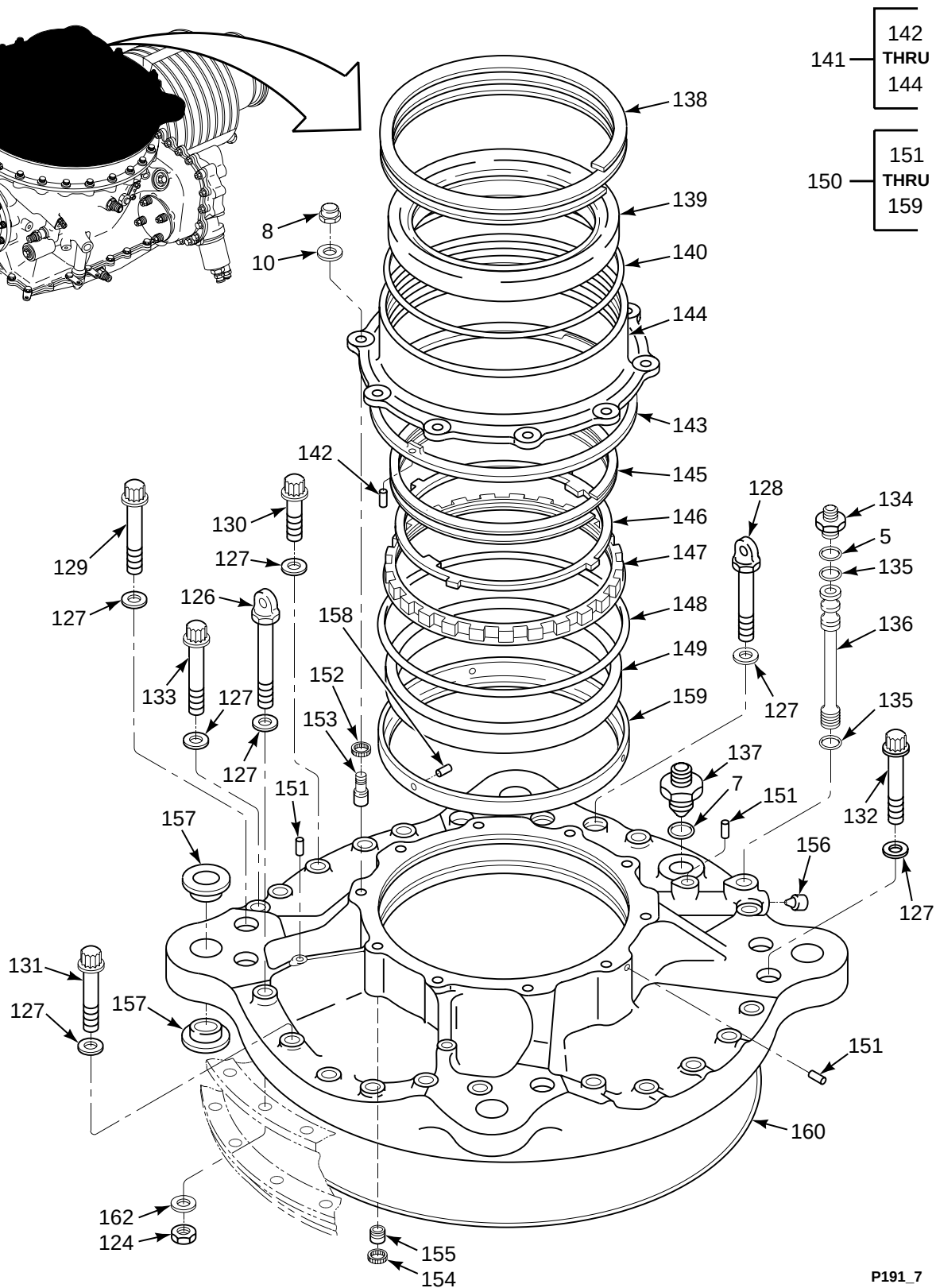
FIGURE 191. TRANSMISSION, AFT (SHEET 7 OF 13)
