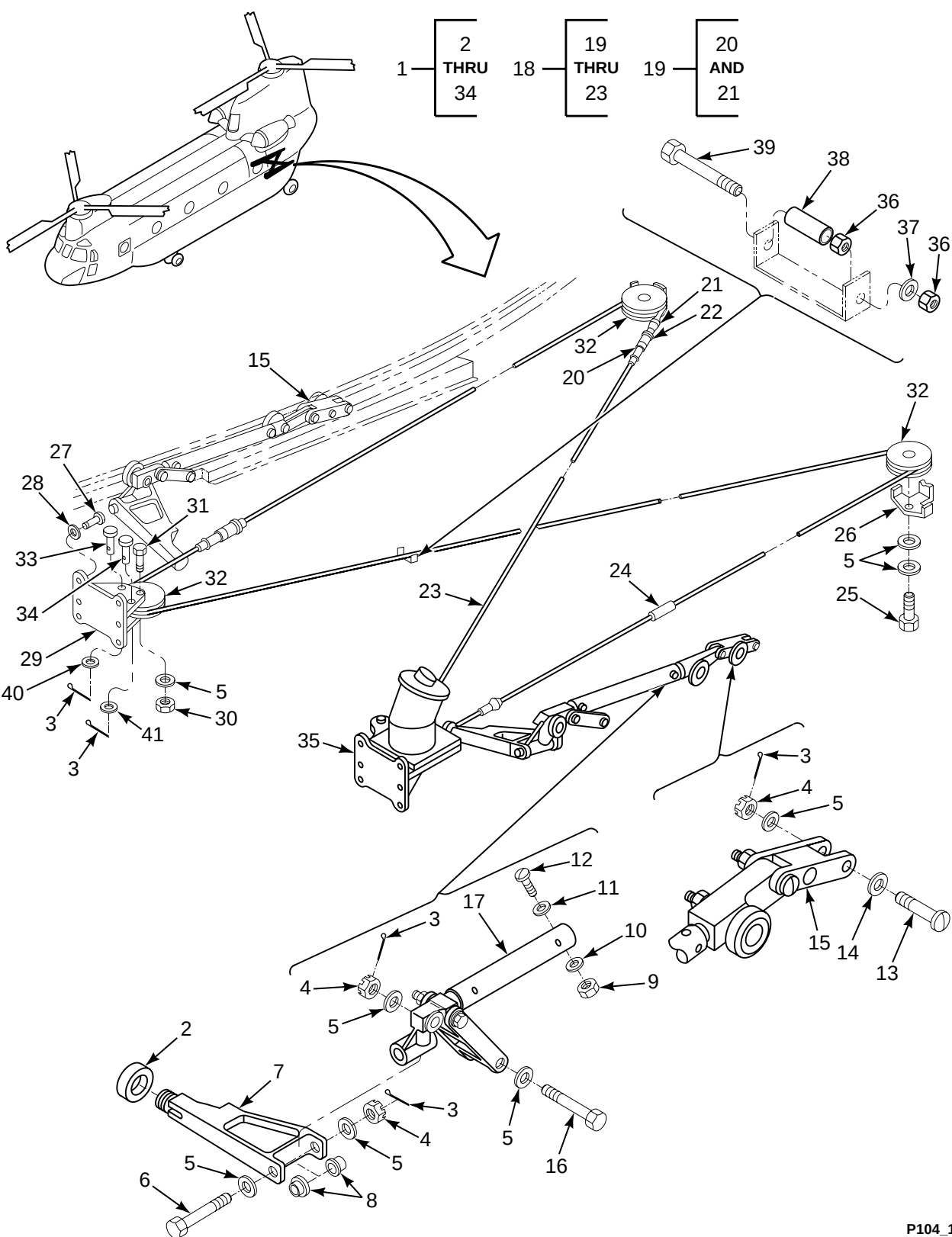
FIGURE 104. MECHANISM INSTL, CARGO DOOR
