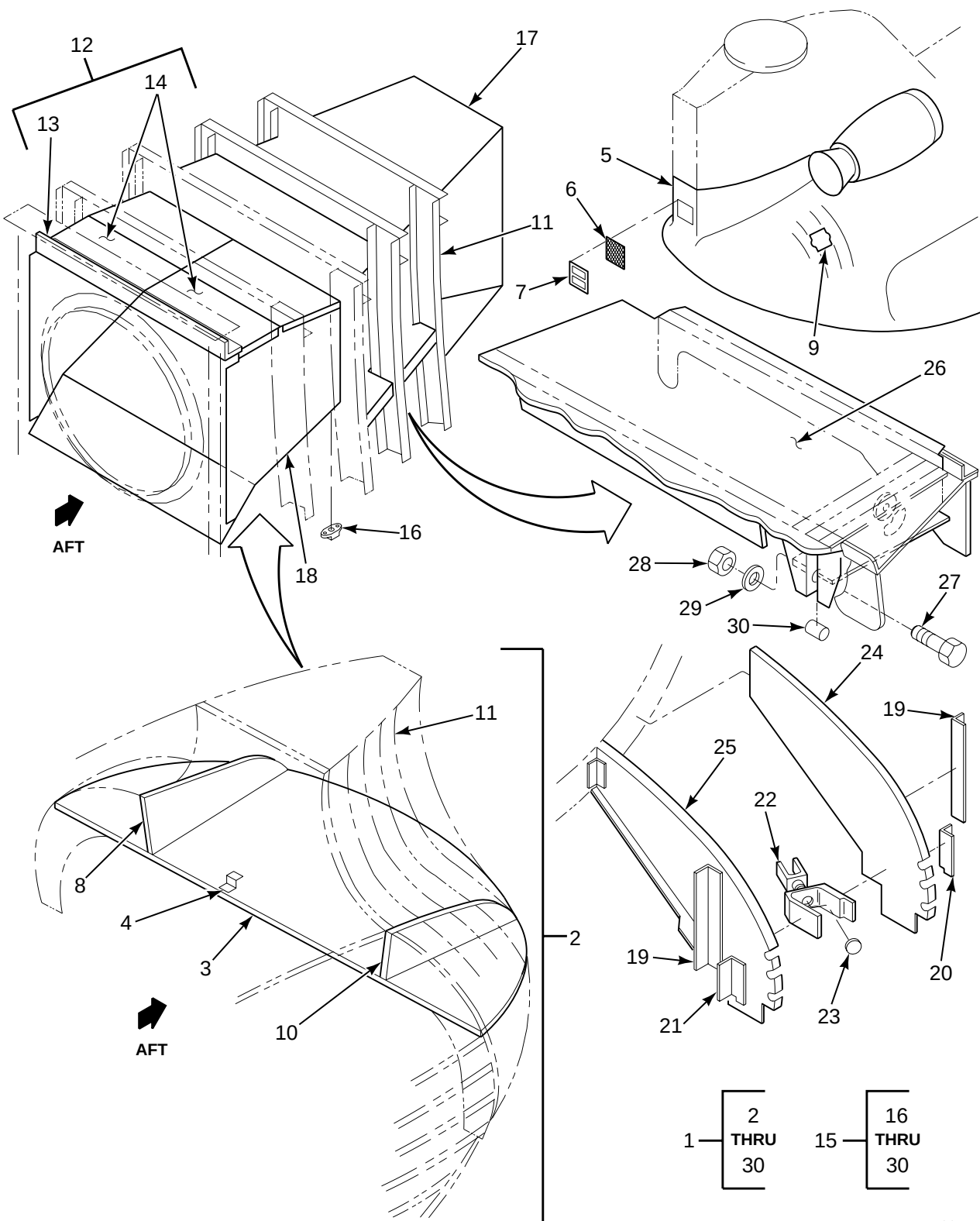
FIGURE 120. TAILCONE INSTL
