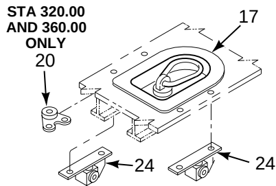
DETAIL G
