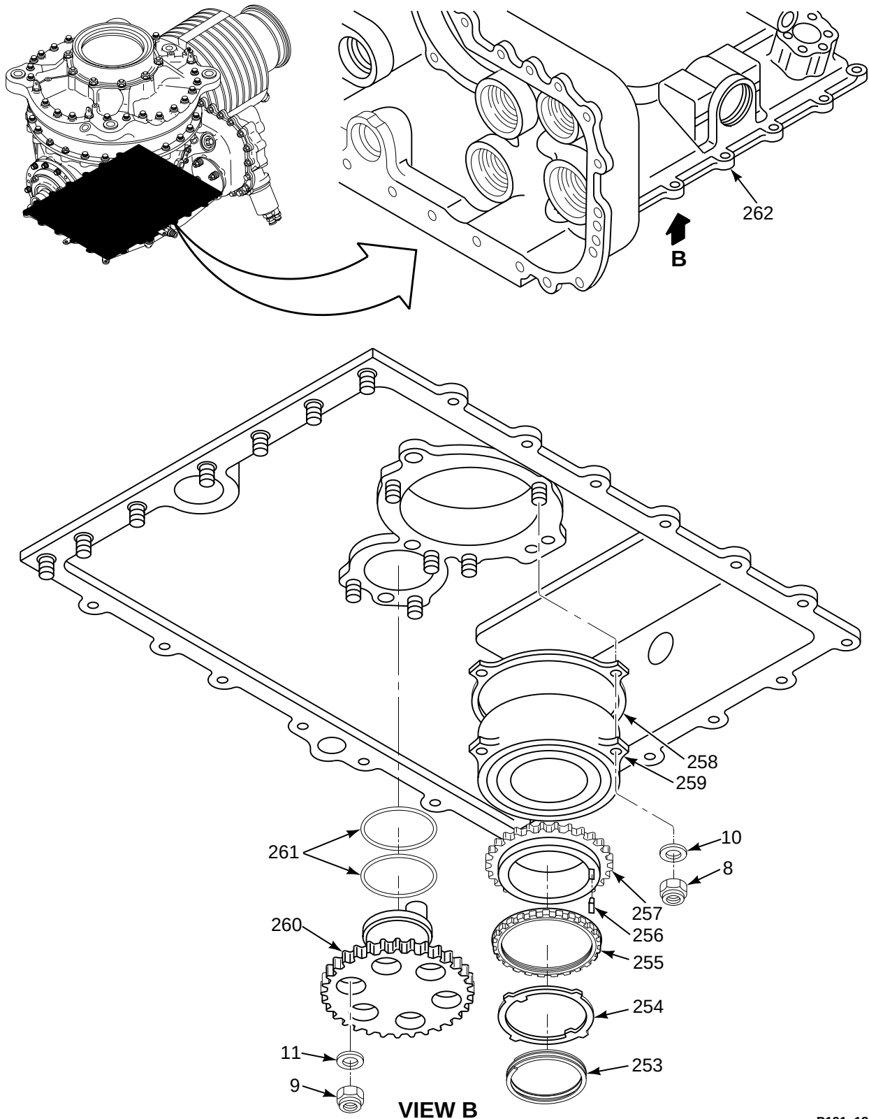
FIGURE 191. TRANSMISSION, AFT (SHEET 13 OF 13)
