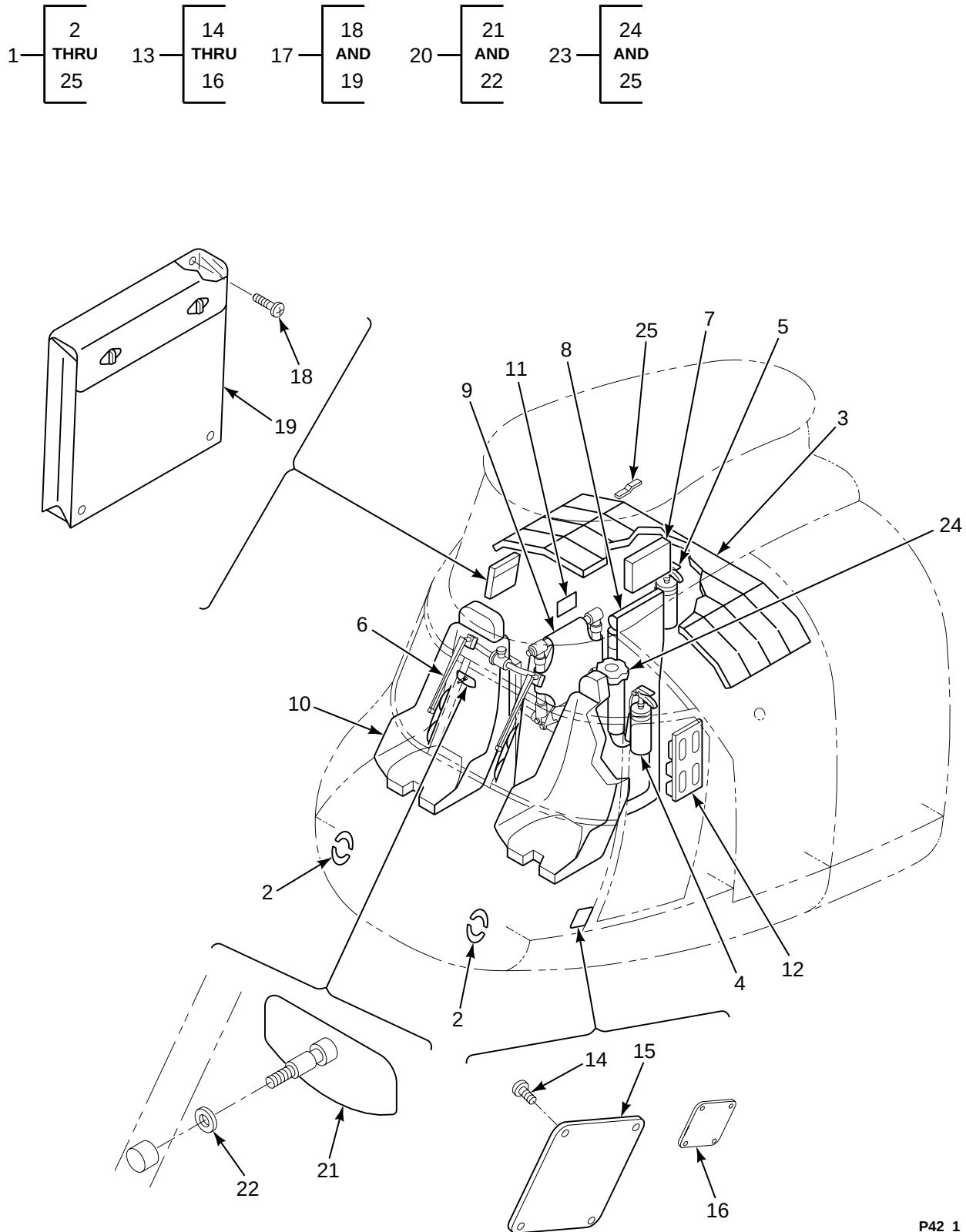
FIGURE 42. EQUIPMENT INSTL, COCKPIT
