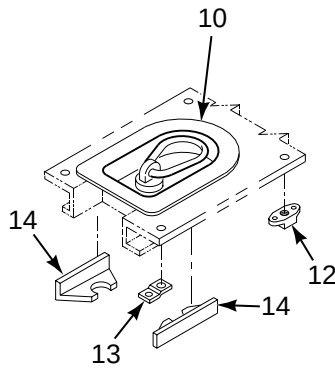
DETAIL E
