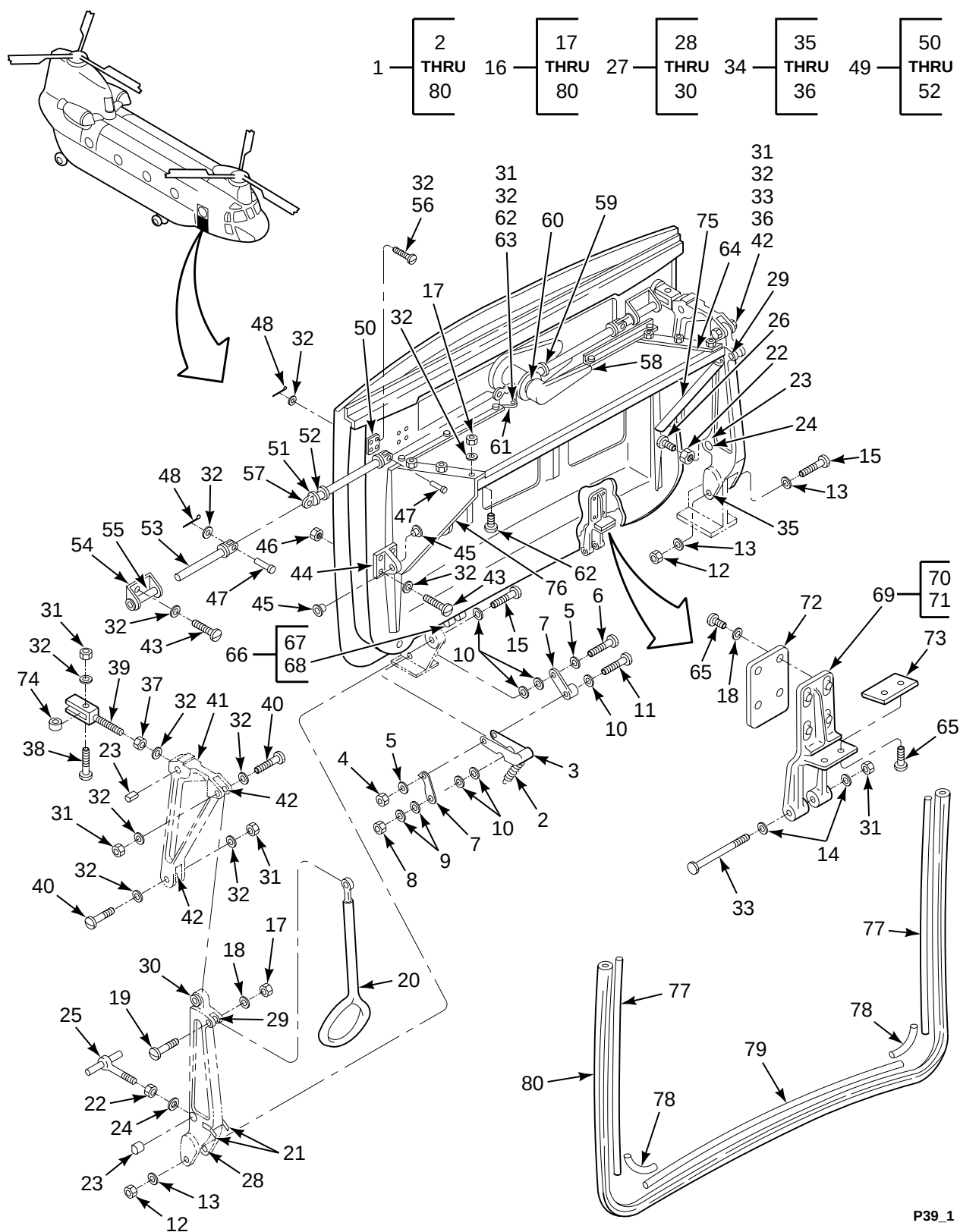
FIGURE 39. DOOR INSTL, CABIN, LOWER
