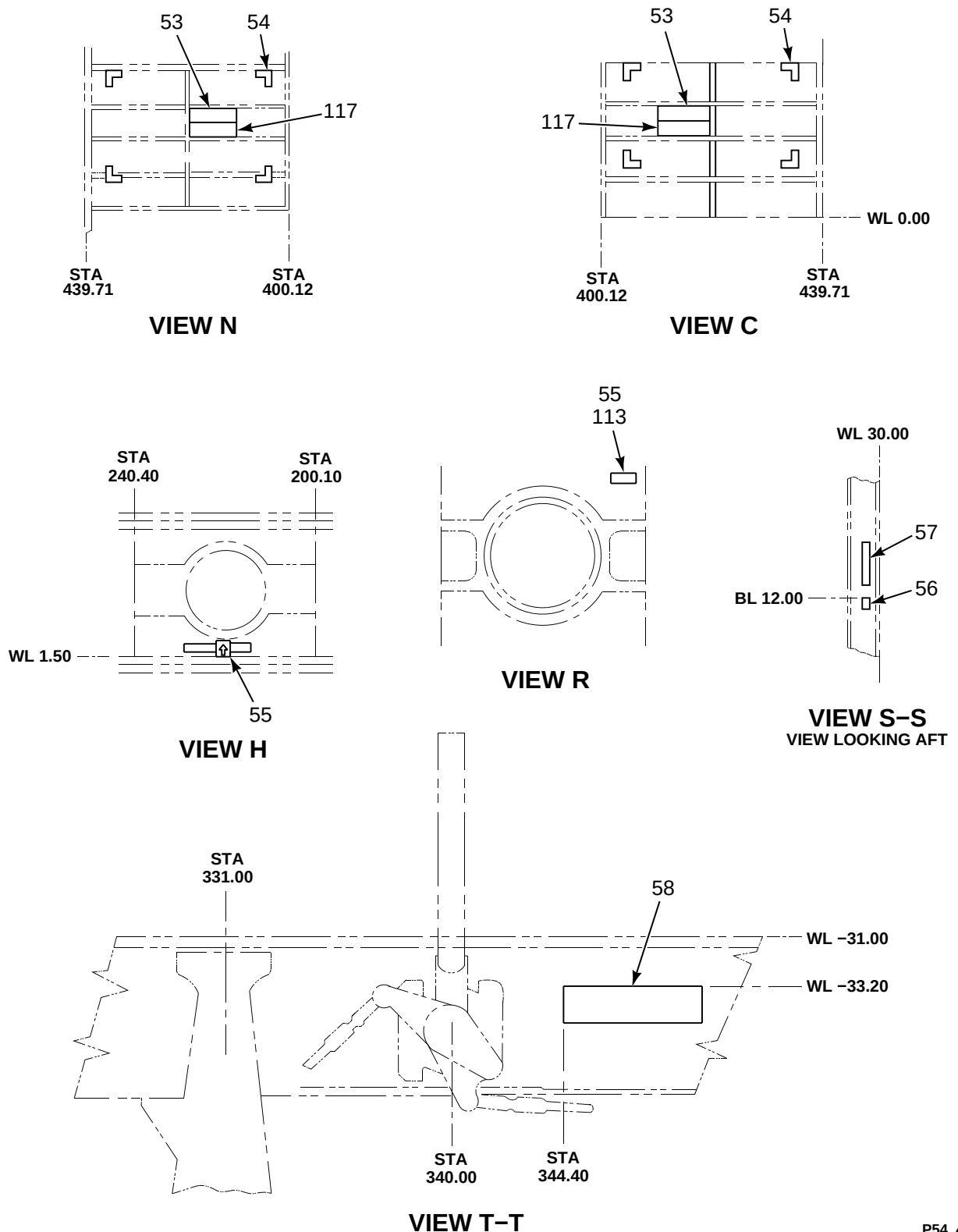
FIGURE 54. MARKINGS, INTERIOR (SHEET 4 OF 8)
