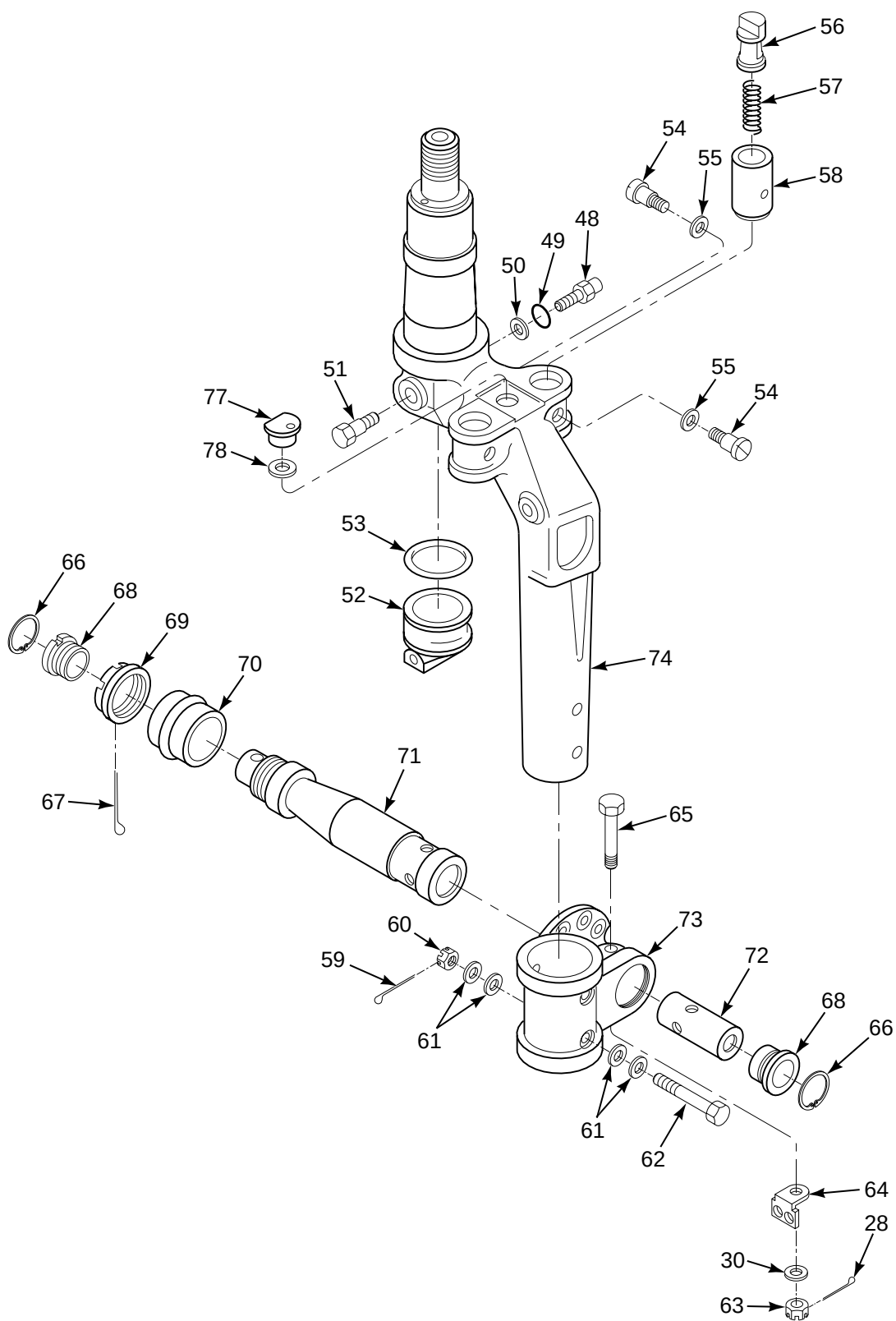
FIGURE 152. HOUSING, SWIVEL, AFT LANDING GEAR (SHEET 2 OF 2)
