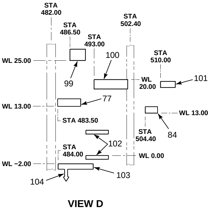
FIGURE 54. MARKINGS, INTERIOR (SHEET 7 OF 8)
