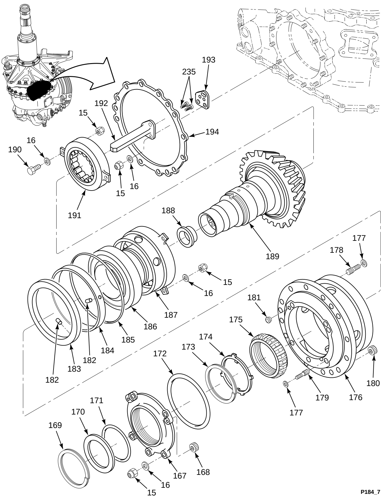
FIGURE 184. TRANSMISSION, FWD (SHEET 7 OF 9)
