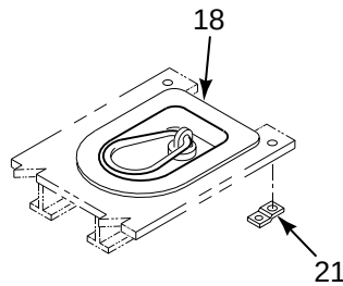
DETAIL H
