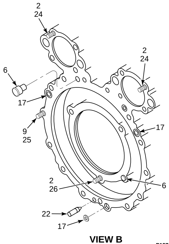
FIGURE 197. HOUSING, MAIN COMBINING TRANSMISSION (SHEET 2 OF 2)
